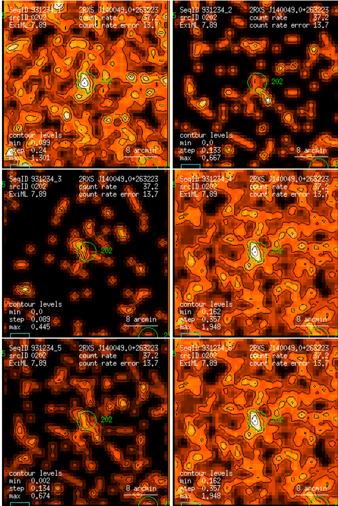
Figure 202: RASS 931234: detection 0202: band rate images, Gaussian filter: (1) PSPC channels 11 – 41, (2) 52 – 90, (3) 91 – 201, (4) 11 – 235, (5) 52 – 201, (6) 11 – 201. Broad band rates in counts/ks. Band rate contour levels in counts/ks/arcmin 2 .
