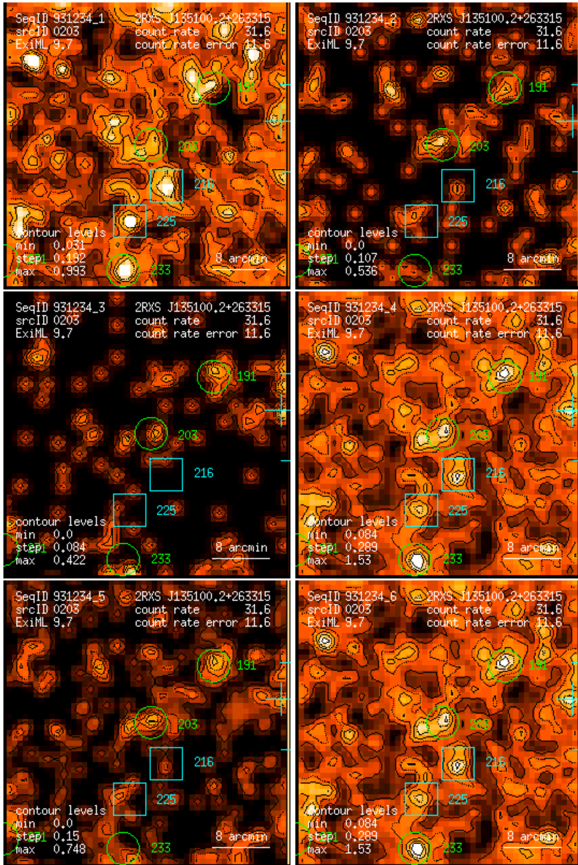
Figure 203: RASS 931234: detection 0203: band rate images, Gaussian filter: (1) PSPC channels 11 – 41, (2) 52 – 90, (3) 91 – 201, (4) 11 – 235, (5) 52 – 201, (6) 11 – 201. Broad band rates in counts/ks. Band rate contour levels in counts/ks/arcmin 2 .
