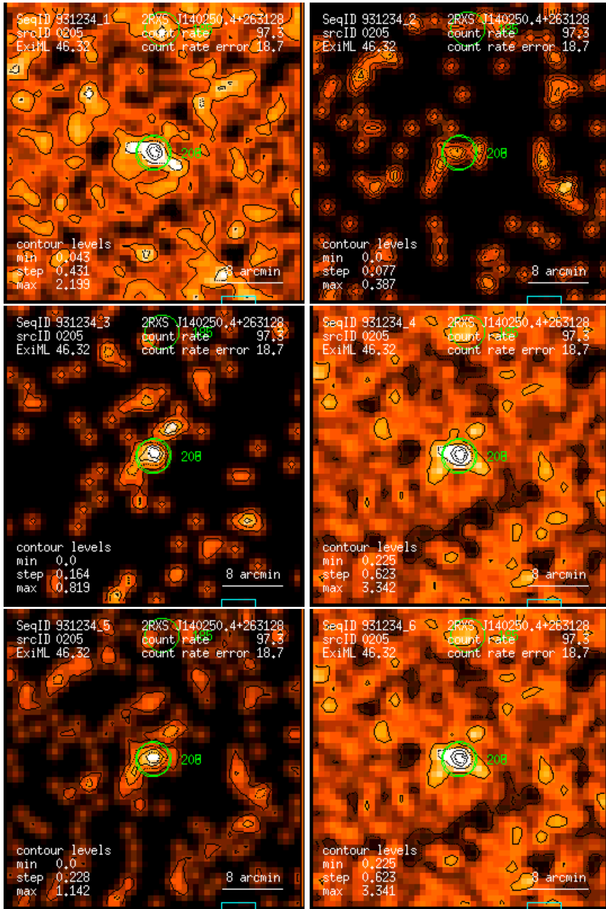
Figure 205: RASS 931234: detection 0205: band rate images, Gaussian filter: (1) PSPC channels 11 – 41, (2) 52 – 90, (3) 91 – 201, (4) 11 – 235, (5) 52 – 201, (6) 11 – 201. Broad band rates in counts/ks. Band rate contour levels in counts/ks/arcmin 2 .
