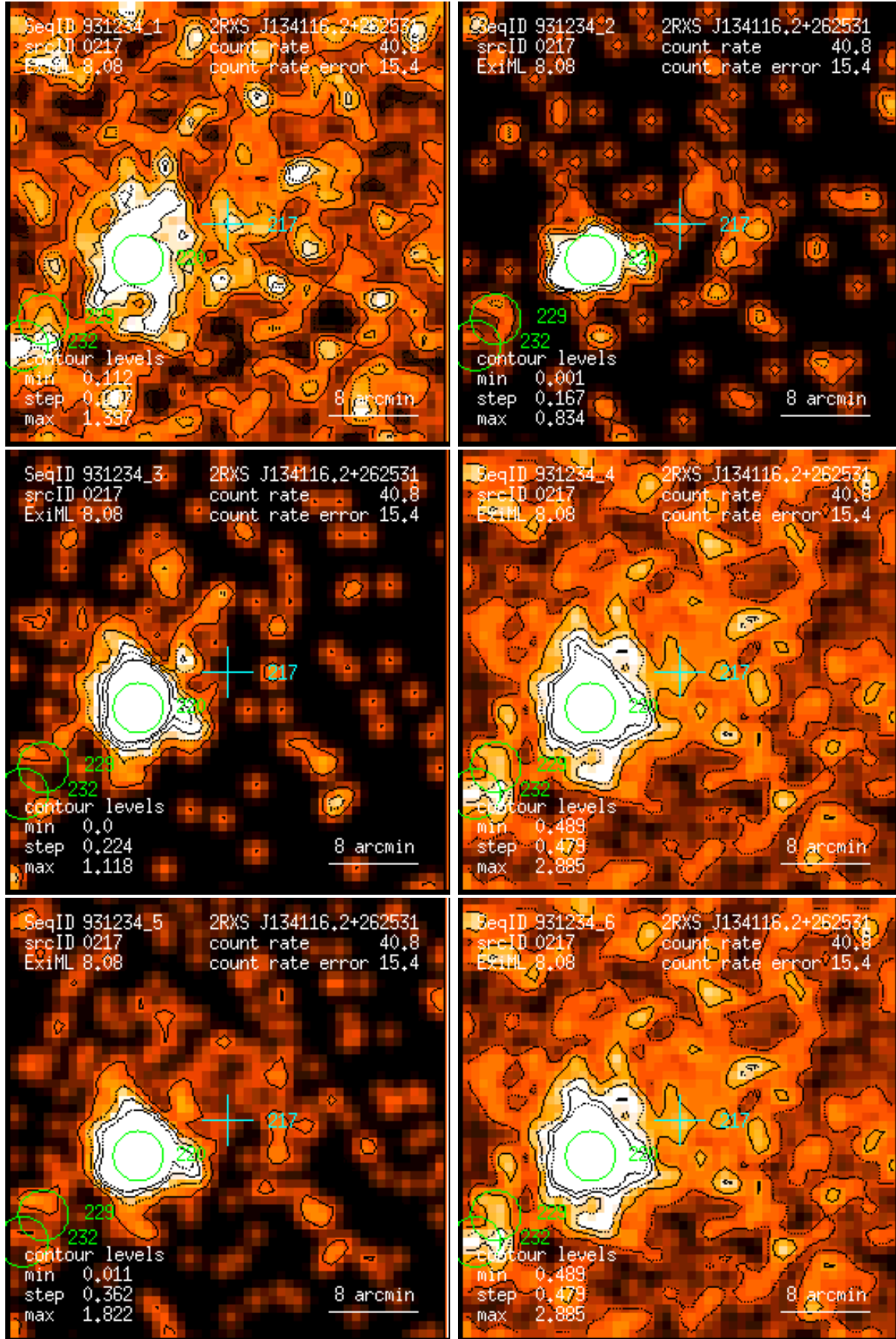
Figure 217: RASS 931234: detection 0217: band rate images, Gaussian filter: (1) PSPC channels 11 – 41, (2) 52 – 90, (3) 91 – 201, (4) 11 – 235, (5) 52 – 201, (6) 11 – 201. Broad band rates in counts/ks. Band rate contour levels in counts/ks/arcmin 2 .
