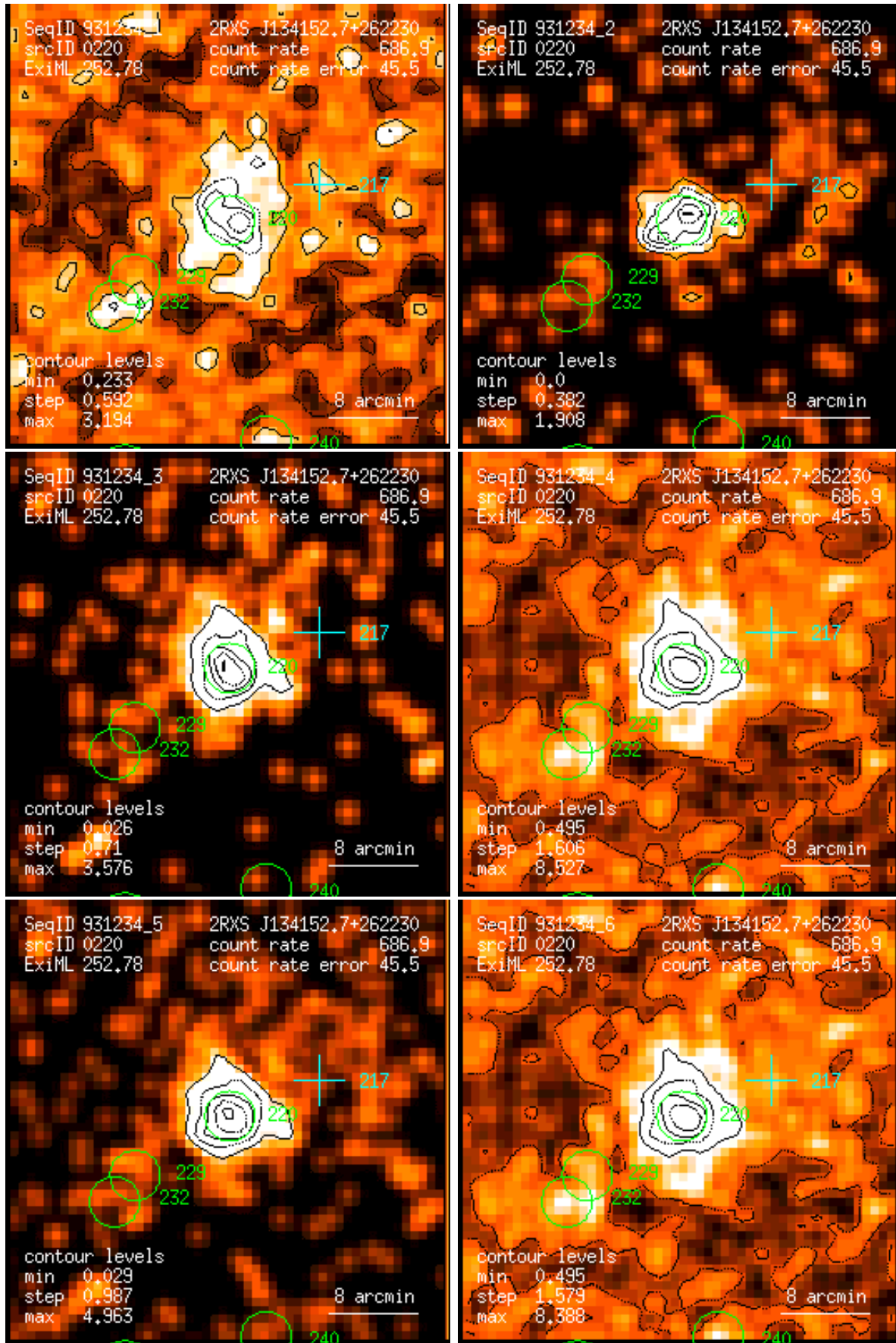
Figure 220: RASS 931234: detection 0220: band rate images, Gaussian filter: (1) PSPC channels 11 – 41, (2) 52 – 90, (3) 91 – 201, (4) 11 – 235, (5) 52 – 201, (6) 11 – 201. Broad band rates in counts/ks. Band rate contour levels in counts/ks/arcmin 2 .
