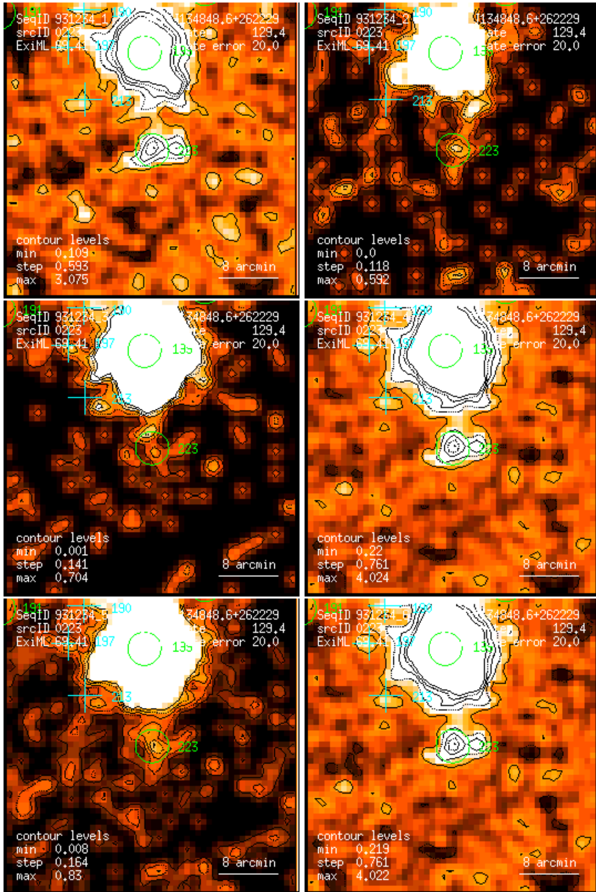
Figure 223: RASS 931234: detection 0223: band rate images, Gaussian filter: (1) PSPC channels 11 – 41, (2) 52 – 90, (3) 91 – 201, (4) 11 – 235, (5) 52 – 201, (6) 11 – 201. Broad band rates in counts/ks. Band rate contour levels in counts/ks/arcmin 2 .
