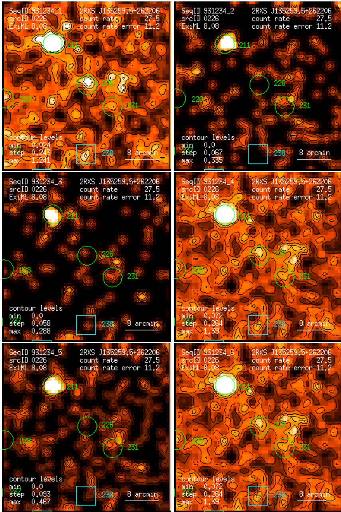
Figure 226: RASS 931234: detection 0226: band rate images, Gaussian filter: (1) PSPC channels 11 – 41, (2) 52 – 90, (3) 91 – 201, (4) 11 – 235, (5) 52 – 201, (6) 11 – 201. Broad band rates in counts/ks. Band rate contour levels in counts/ks/arcmin 2 .
