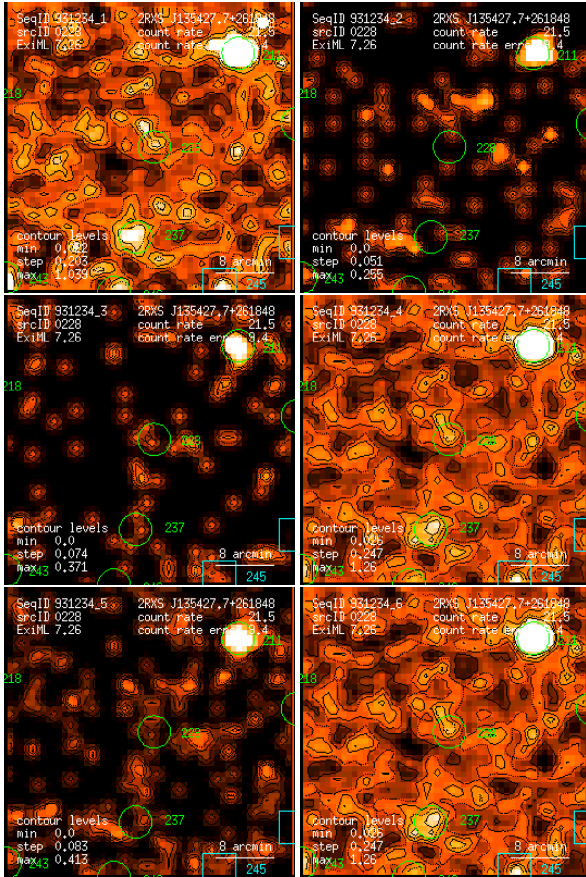
Figure 228: RASS 931234: detection 0228: band rate images, Gaussian filter: (1) PSPC channels 11 – 41, (2) 52 – 90, (3) 91 – 201, (4) 11 – 235, (5) 52 – 201, (6) 11 – 201. Broad band rates in counts/ks. Band rate contour levels in counts/ks/arcmin 2 .
