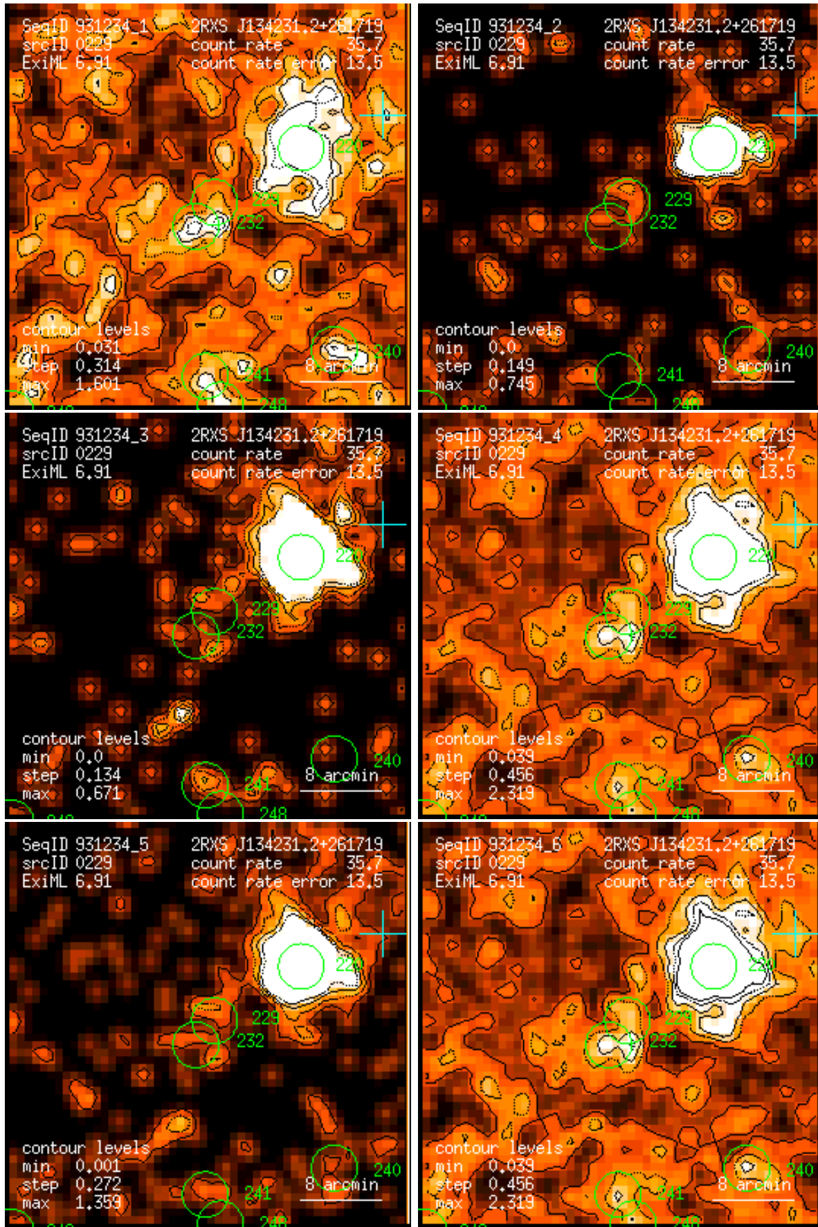
Figure 229: RASS 931234: detection 0229: band rate images, Gaussian filter: (1) PSPC channels 11 – 41, (2) 52 – 90, (3) 91 – 201, (4) 11 – 235, (5) 52 – 201, (6) 11 – 201. Broad band rates in counts/ks. Band rate contour levels in counts/ks/arcmin 2 .
