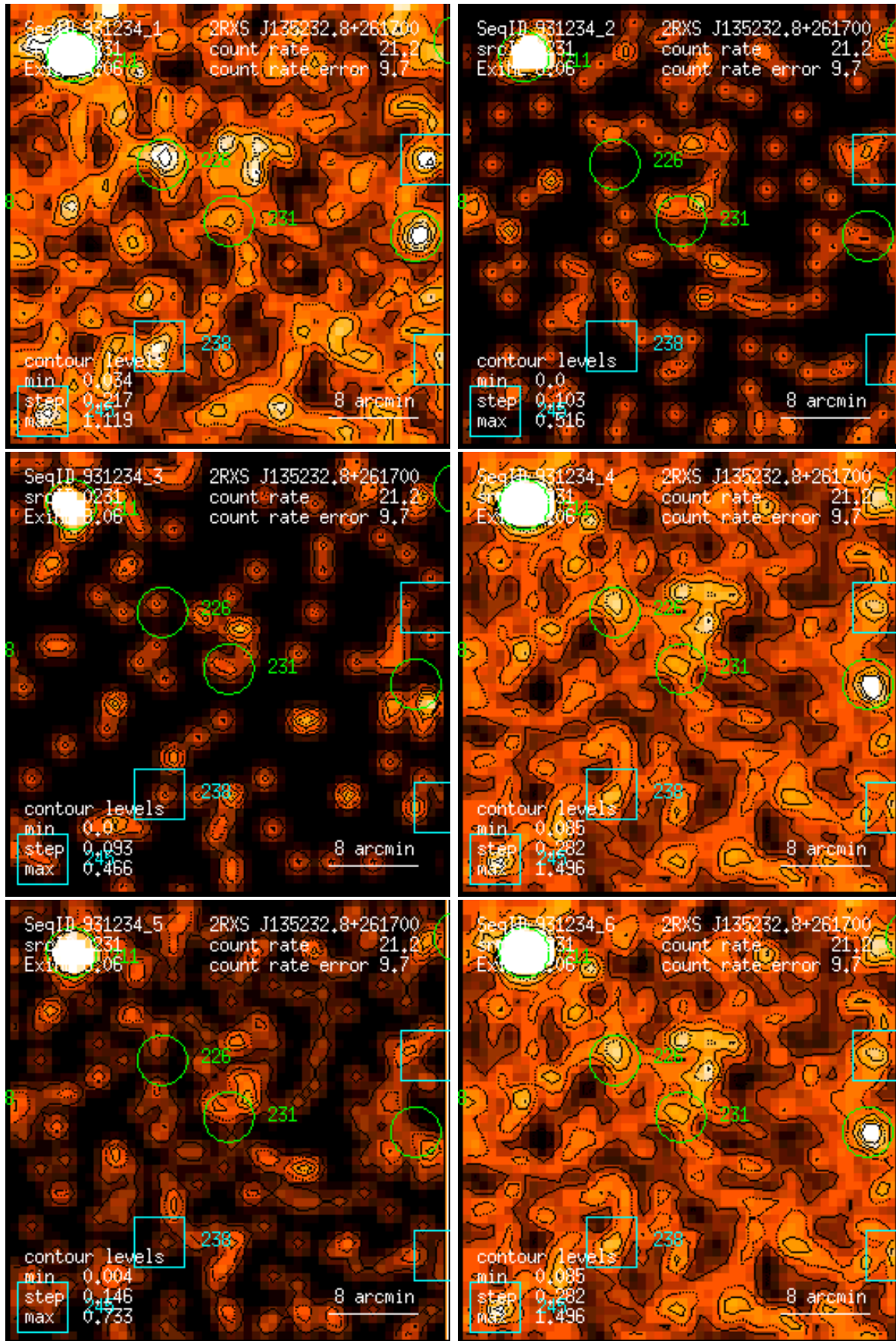
Figure 231: RASS 931234: detection 0231: band rate images, Gaussian filter: (1) PSPC channels 11 – 41, (2) 52 – 90, (3) 91 – 201, (4) 11 – 235, (5) 52 – 201, (6) 11 – 201. Broad band rates in counts/ks. Band rate contour levels in counts/ks/arcmin 2 .
