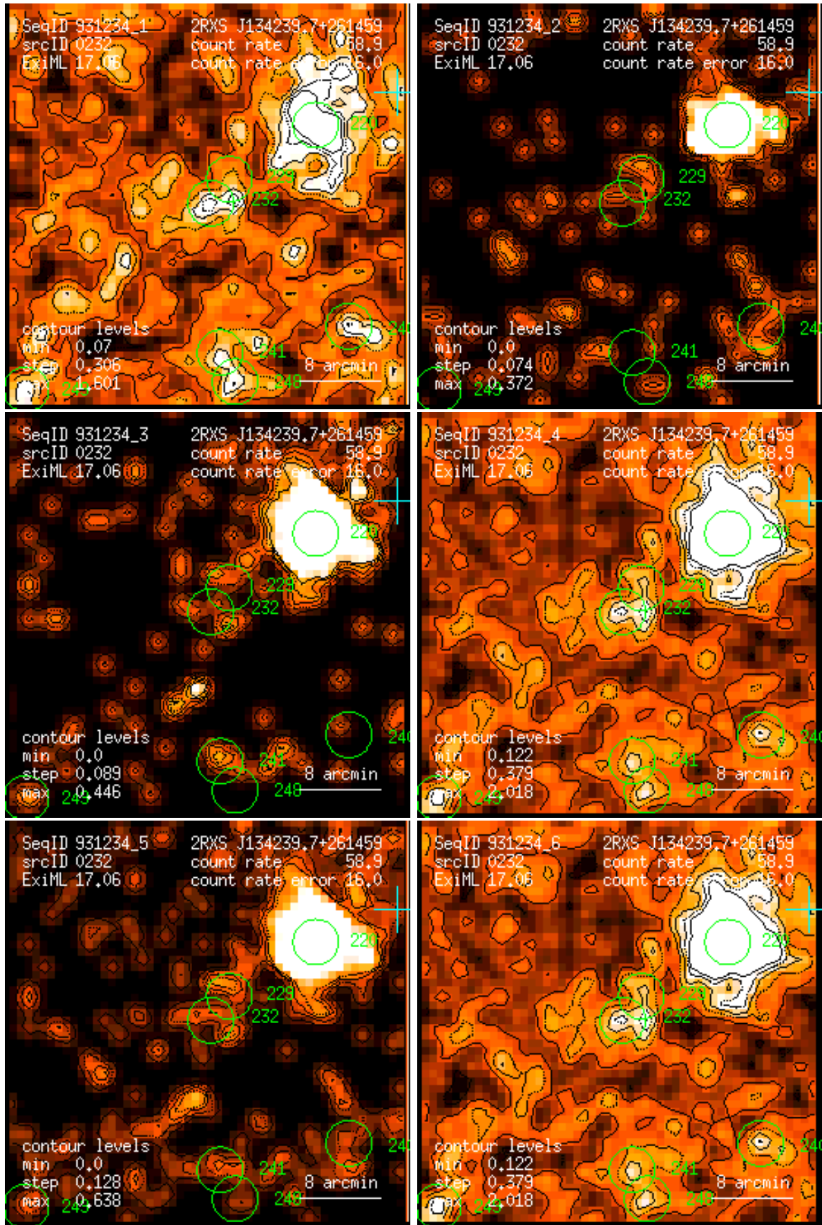
Figure 232: RASS 931234: detection 0232: band rate images, Gaussian filter: (1) PSPC channels 11 – 41, (2) 52 – 90, (3) 91 – 201, (4) 11 – 235, (5) 52 – 201, (6) 11 – 201. Broad band rates in counts/ks. Band rate contour levels in counts/ks/arcmin 2 .
