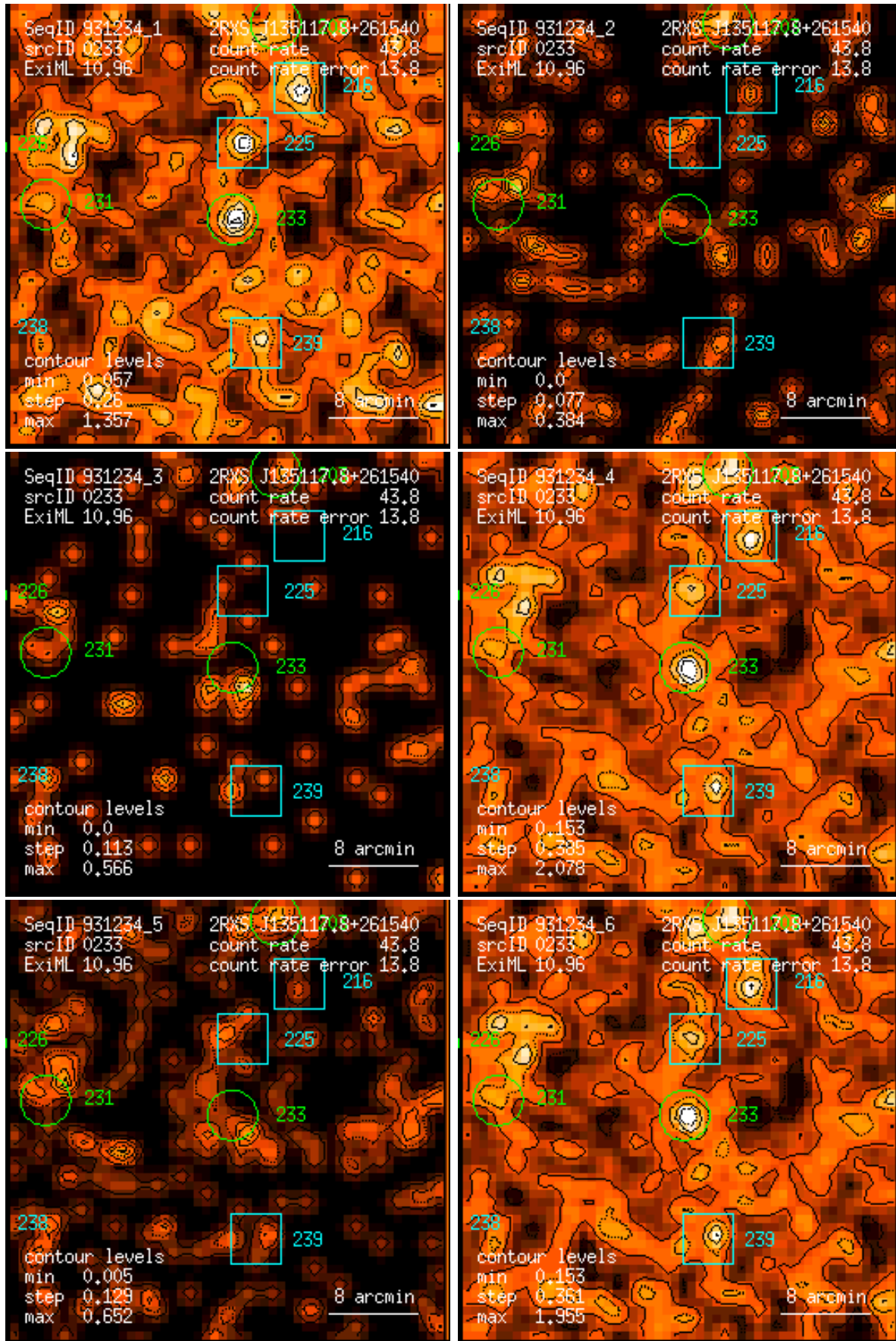
Figure 233: RASS 931234: detection 0233: band rate images, Gaussian filter: (1) PSPC channels 11 – 41, (2) 52 – 90, (3) 91 – 201, (4) 11 – 235, (5) 52 – 201, (6) 11 – 201. Broad band rates in counts/ks. Band rate contour levels in counts/ks/arcmin 2 .
