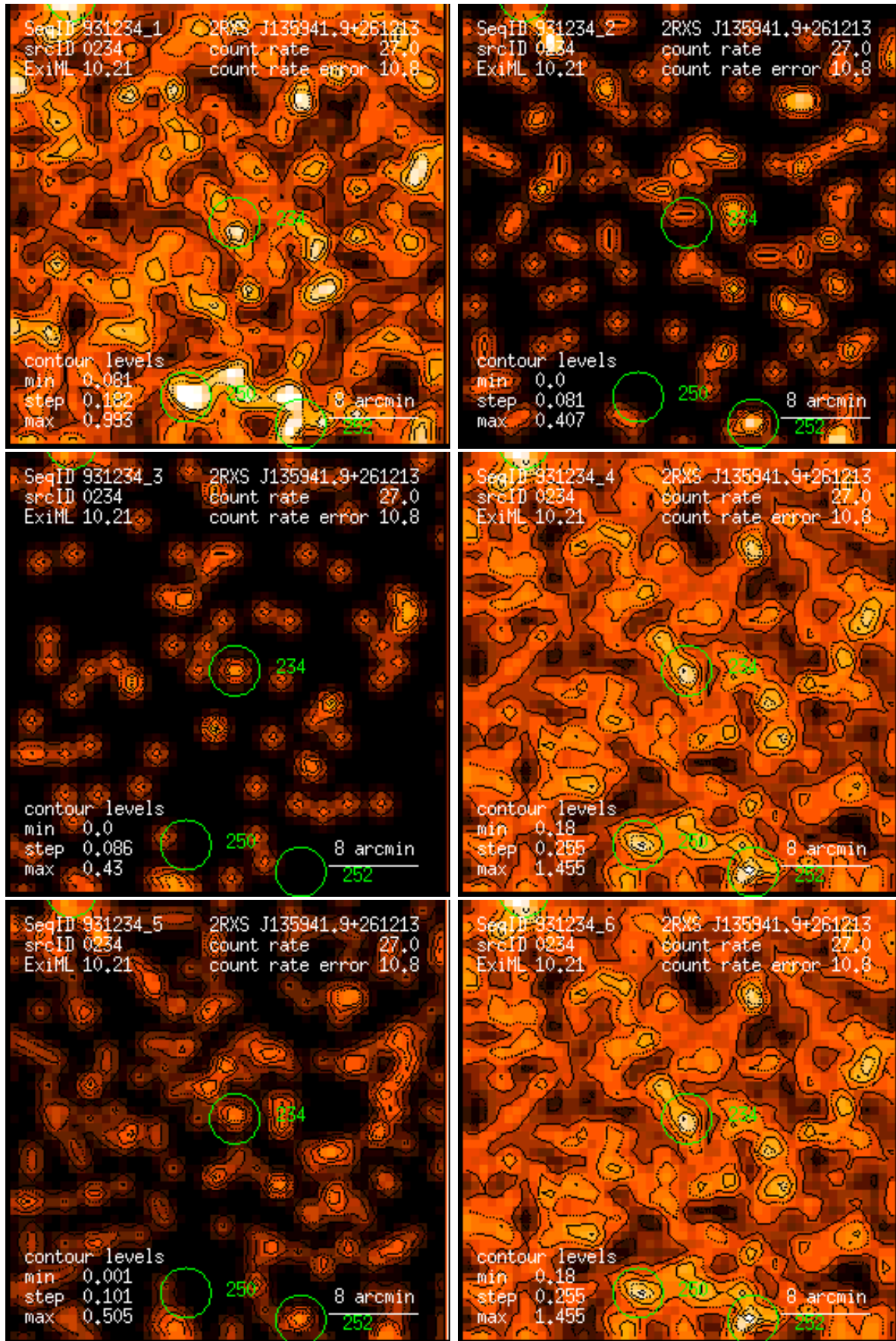
Figure 234: RASS 931234: detection 0234: band rate images, Gaussian filter: (1) PSPC channels 11 – 41, (2) 52 – 90, (3) 91 – 201, (4) 11 – 235, (5) 52 – 201, (6) 11 – 201. Broad band rates in counts/ks. Band rate contour levels in counts/ks/arcmin 2 .
