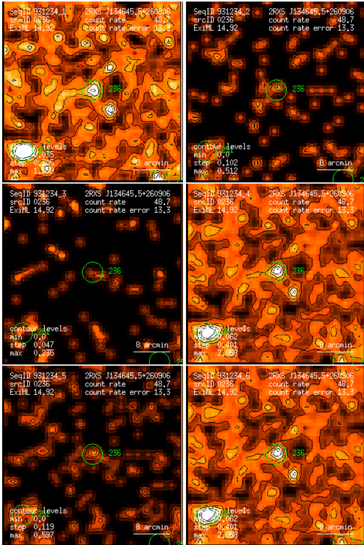
Figure 236: RASS 931234: detection 0236: band rate images, Gaussian filter: (1) PSPC channels 11 – 41, (2) 52 – 90, (3) 91 – 201, (4) 11 – 235, (5) 52 – 201, (6) 11 – 201. Broad band rates in counts/ks. Band rate contour levels in counts/ks/arcmin 2 .
