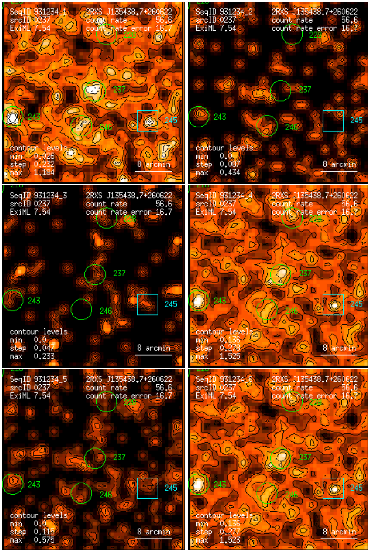
Figure 237: RASS 931234: detection 0237: band rate images, Gaussian filter: (1) PSPC channels 11 – 41, (2) 52 – 90, (3) 91 – 201, (4) 11 – 235, (5) 52 – 201, (6) 11 – 201. Broad band rates in counts/ks. Band rate contour levels in counts/ks/arcmin 2 .
