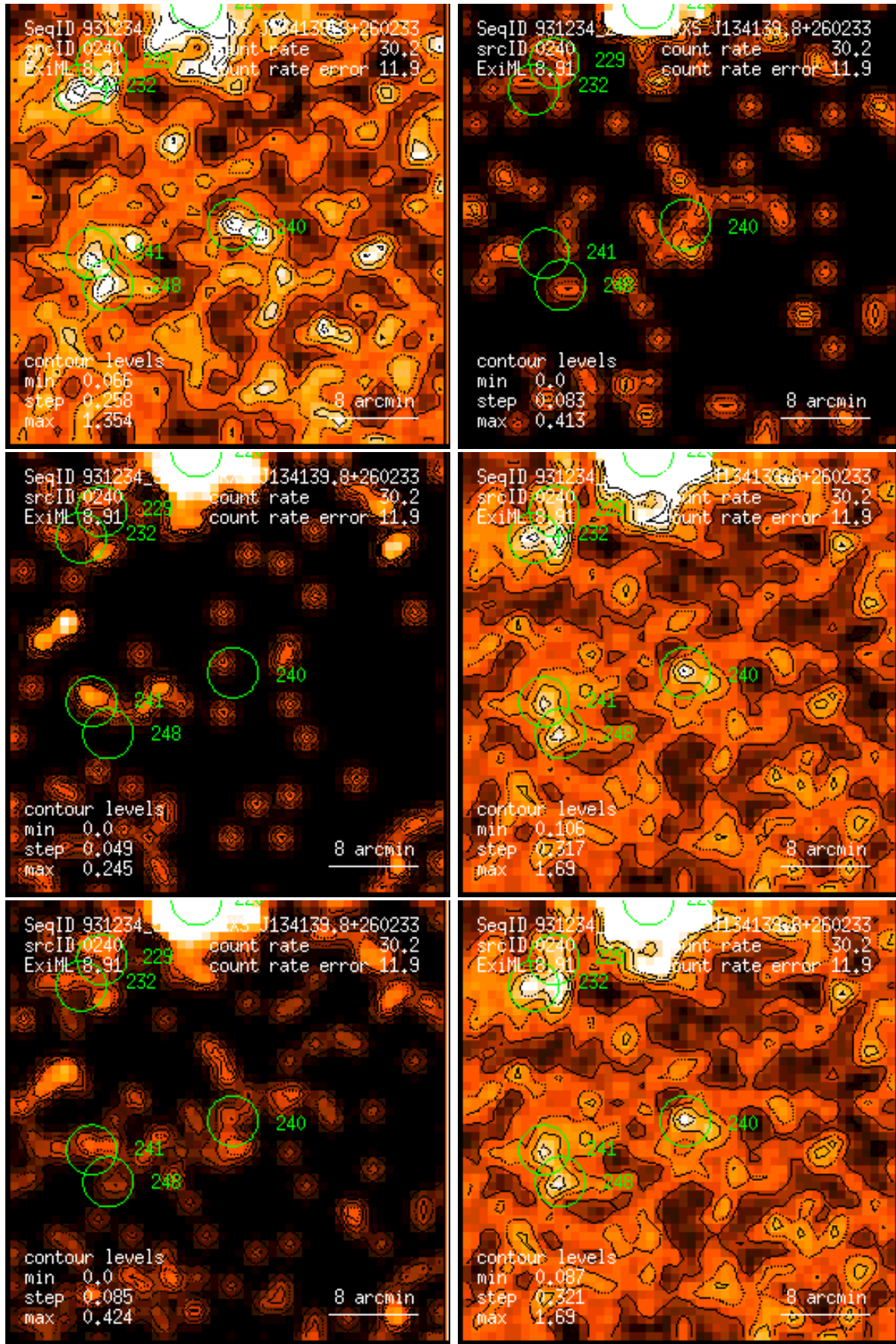
Figure 240: RASS 931234: detection 0240: band rate images, Gaussian filter: (1) PSPC channels 11 – 41, (2) 52 – 90, (3) 91 – 201, (4) 11 – 235, (5) 52 – 201, (6) 11 – 201. Broad band rates in counts/ks. Band rate contour levels in counts/ks/arcmin 2 .
