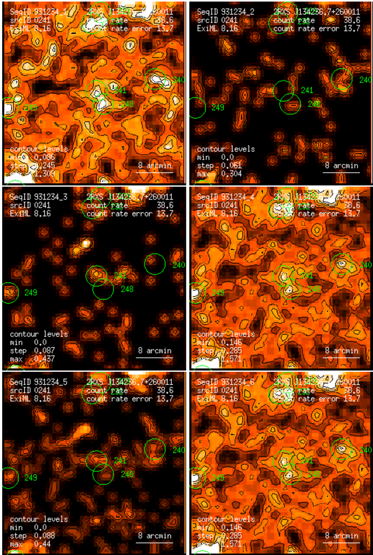
Figure 241: RASS 931234: detection 0241: band rate images, Gaussian filter: (1) PSPC channels 11 – 41, (2) 52 – 90, (3) 91 – 201, (4) 11 – 235, (5) 52 – 201, (6) 11 – 201. Broad band rates in counts/ks. Band rate contour levels in counts/ks/arcmin 2 .
