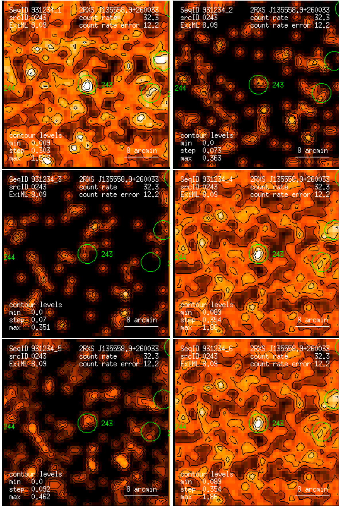
Figure 243: RASS 931234: detection 0243: band rate images, Gaussian filter: (1) PSPC channels 11 – 41, (2) 52 – 90, (3) 91 – 201, (4) 11 – 235, (5) 52 – 201, (6) 11 – 201. Broad band rates in counts/ks. Band rate contour levels in counts/ks/arcmin 2 .
