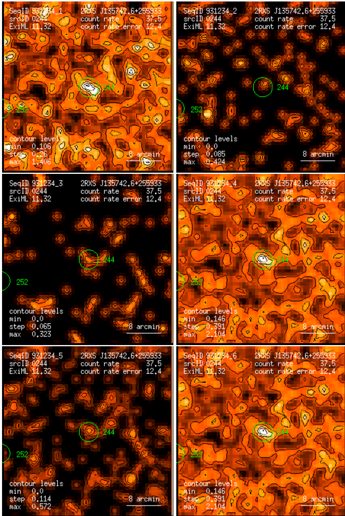
Figure 244: RASS 931234: detection 0244: band rate images, Gaussian filter: (1) PSPC channels 11 – 41, (2) 52 – 90, (3) 91 – 201, (4) 11 – 235, (5) 52 – 201, (6) 11 – 201. Broad band rates in counts/ks. Band rate contour levels in counts/ks/arcmin 2 .
