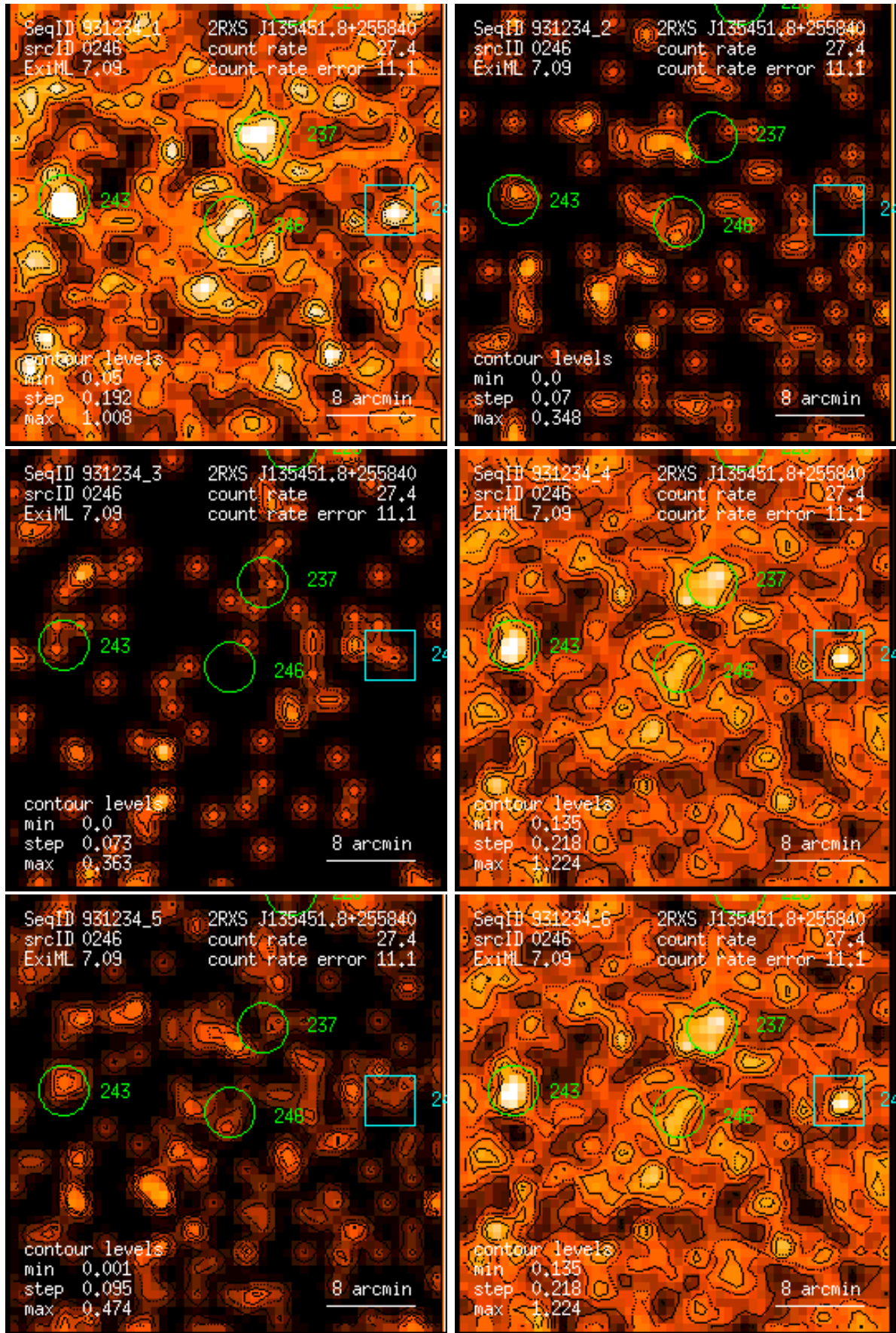
Figure 246: RASS 931234: detection 0246: band rate images, Gaussian filter: (1) PSPC channels 11 – 41, (2) 52 – 90, (3) 91 – 201, (4) 11 – 235, (5) 52 – 201, (6) 11 – 201. Broad band rates in counts/ks. Band rate contour levels in counts/ks/arcmin 2 .
