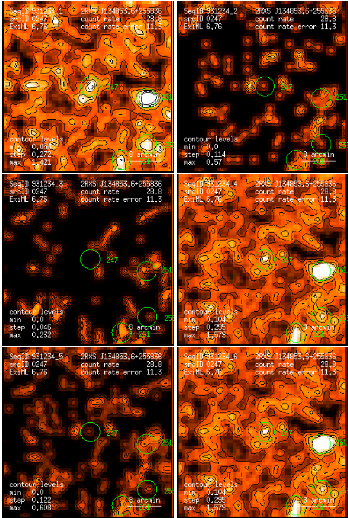
Figure 247: RASS 931234: detection 0247: band rate images, Gaussian filter: (1) PSPC channels 11 – 41, (2) 52 – 90, (3) 91 – 201, (4) 11 – 235, (5) 52 – 201, (6) 11 – 201. Broad band rates in counts/ks. Band rate contour levels in counts/ks/arcmin 2 .
