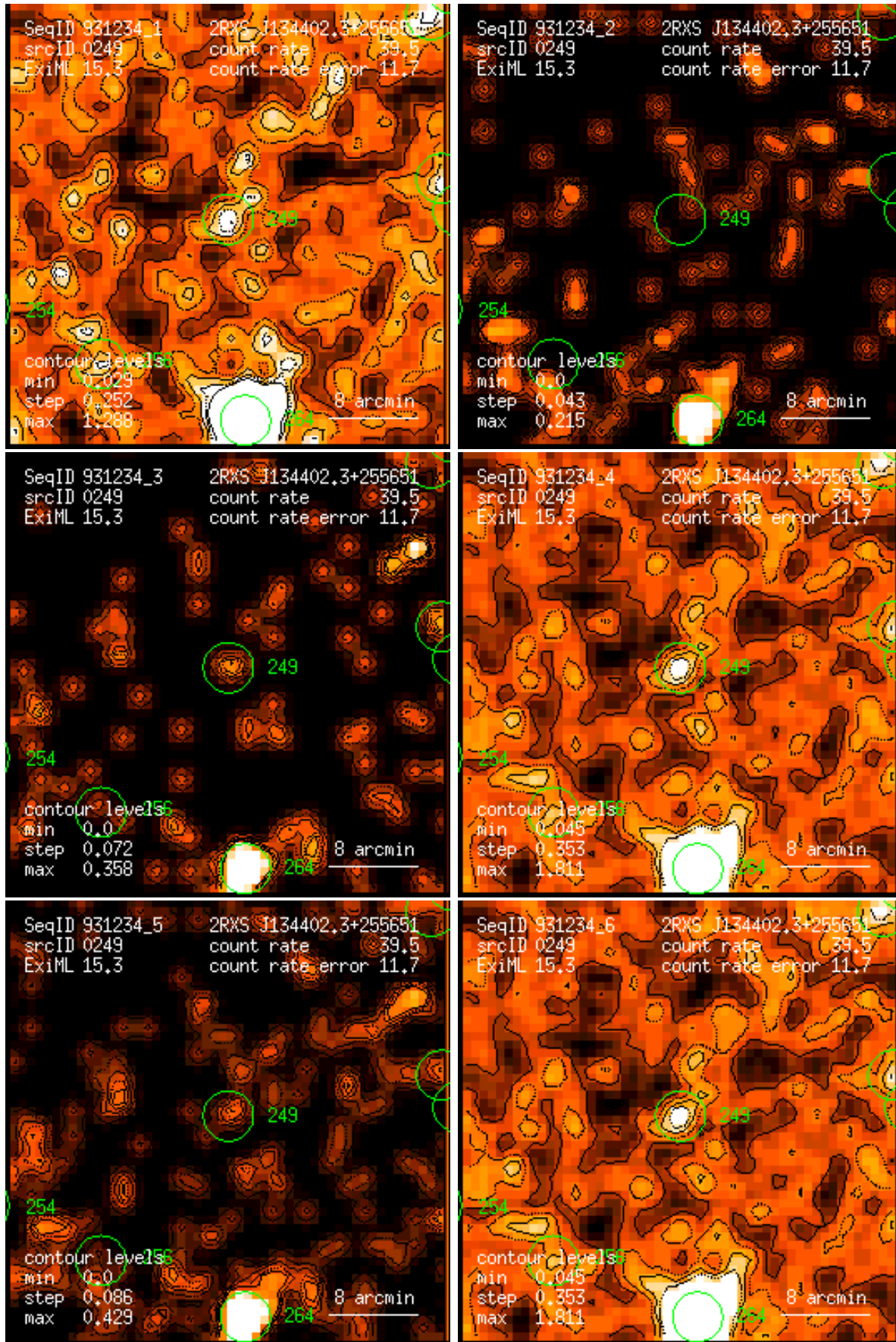
Figure 249: RASS 931234: detection 0249: band rate images, Gaussian filter: (1) PSPC channels 11 – 41, (2) 52 – 90, (3) 91 – 201, (4) 11 – 235, (5) 52 – 201, (6) 11 – 201. Broad band rates in counts/ks. Band rate contour levels in counts/ks/arcmin 2 .
