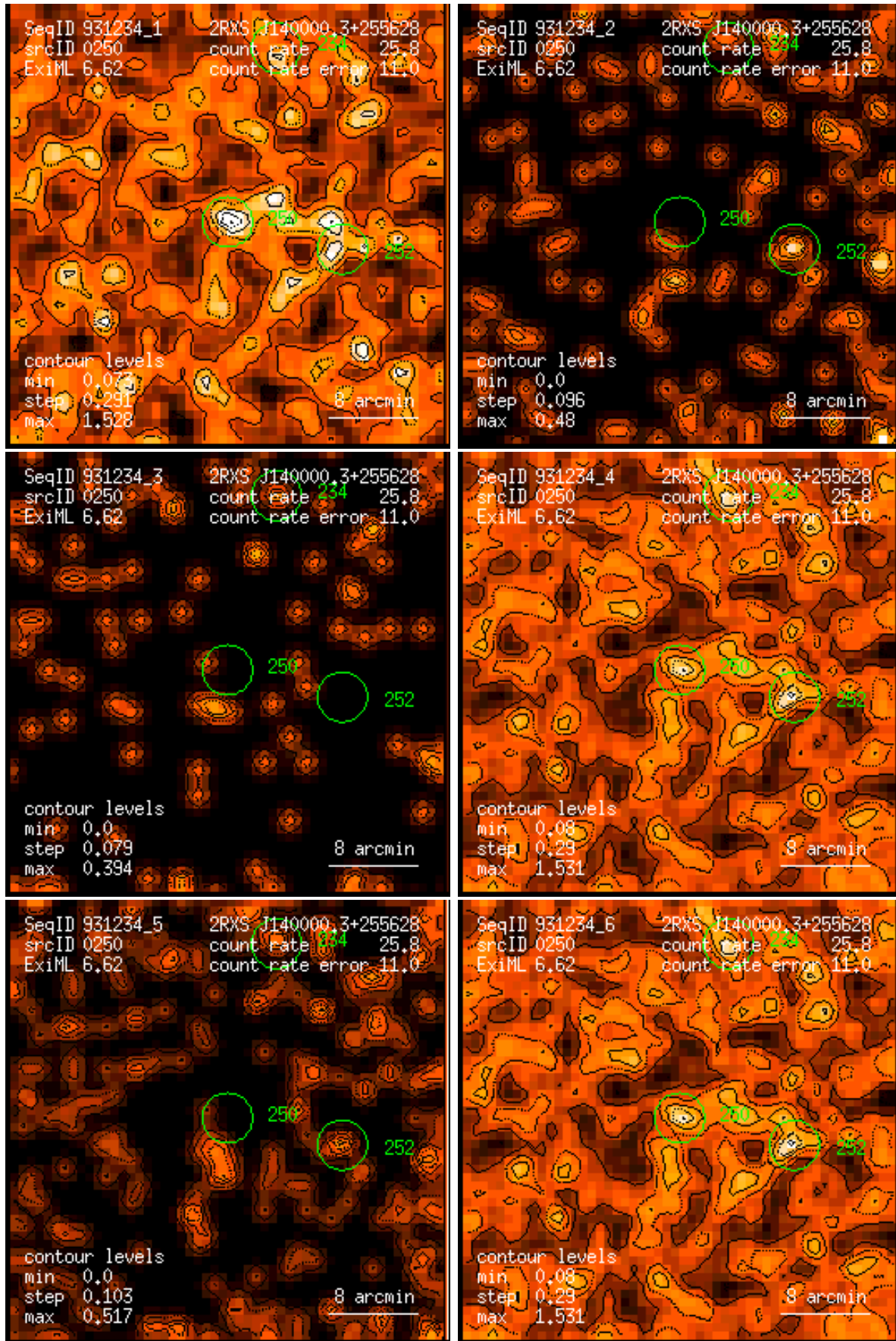
Figure 250: RASS 931234: detection 0250: band rate images, Gaussian filter: (1) PSPC channels 11 – 41, (2) 52 – 90, (3) 91 – 201, (4) 11 – 235, (5) 52 – 201, (6) 11 – 201. Broad band rates in counts/ks. Band rate contour levels in counts/ks/arcmin 2 .
