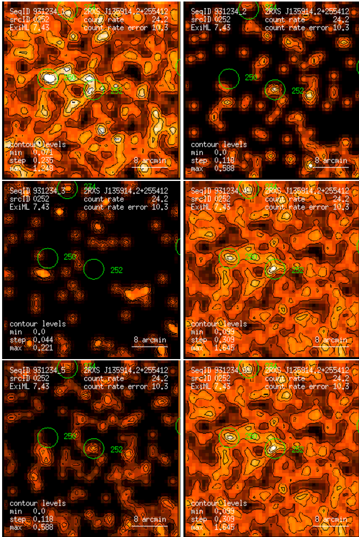
Figure 252: RASS 931234: detection 0252: band rate images, Gaussian filter: (1) PSPC channels 11 – 41, (2) 52 – 90, (3) 91 – 201, (4) 11 – 235, (5) 52 – 201, (6) 11 – 201. Broad band rates in counts/ks. Band rate contour levels in counts/ks/arcmin 2 .
