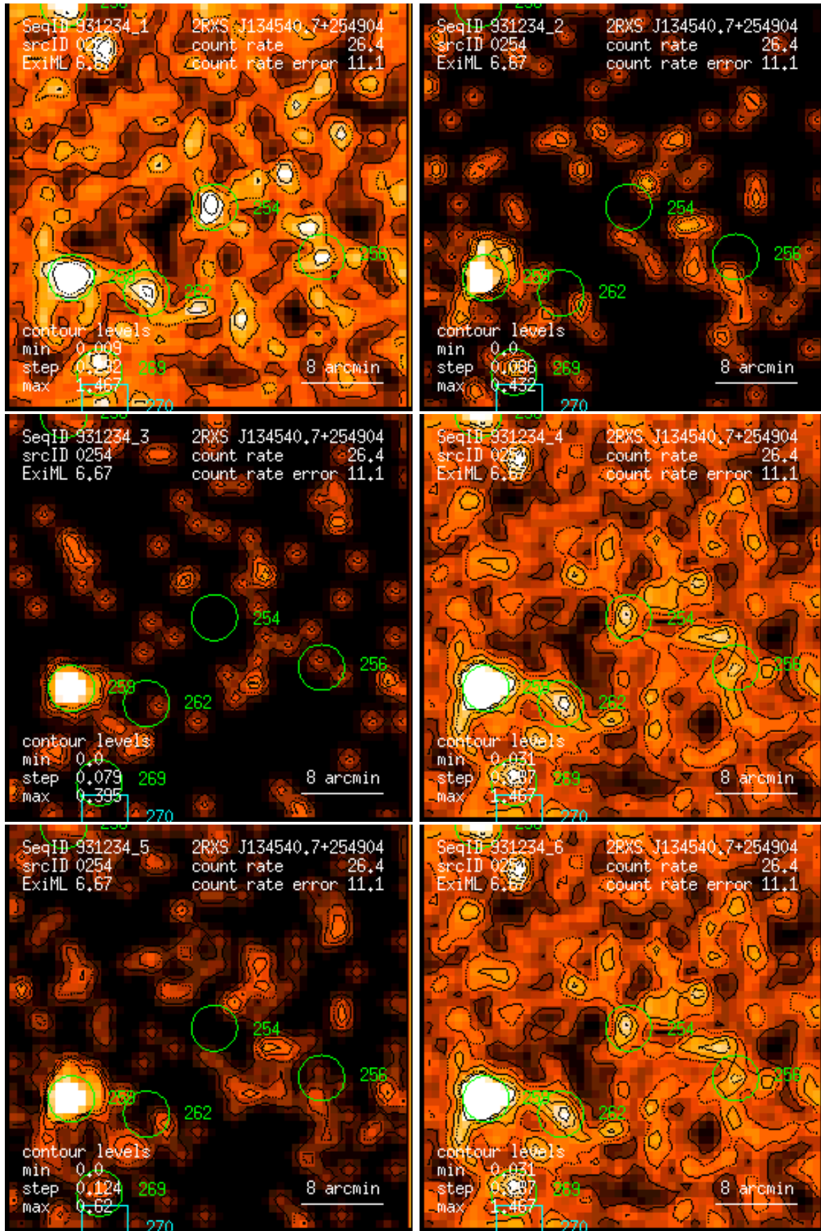
Figure 254: RASS 931234: detection 0254: band rate images, Gaussian filter: (1) PSPC channels 11 – 41, (2) 52 – 90, (3) 91 – 201, (4) 11 – 235, (5) 52 – 201, (6) 11 – 201. Broad band rates in counts/ks. Band rate contour levels in counts/ks/arcmin 2 .
