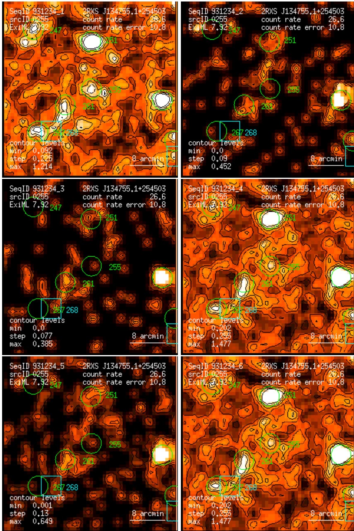
Figure 255: RASS 931234: detection 0255: band rate images, Gaussian filter: (1) PSPC channels 11 – 41, (2) 52 – 90, (3) 91 – 201, (4) 11 – 235, (5) 52 – 201, (6) 11 – 201. Broad band rates in counts/ks. Band rate contour levels in counts/ks/arcmin 2 .
