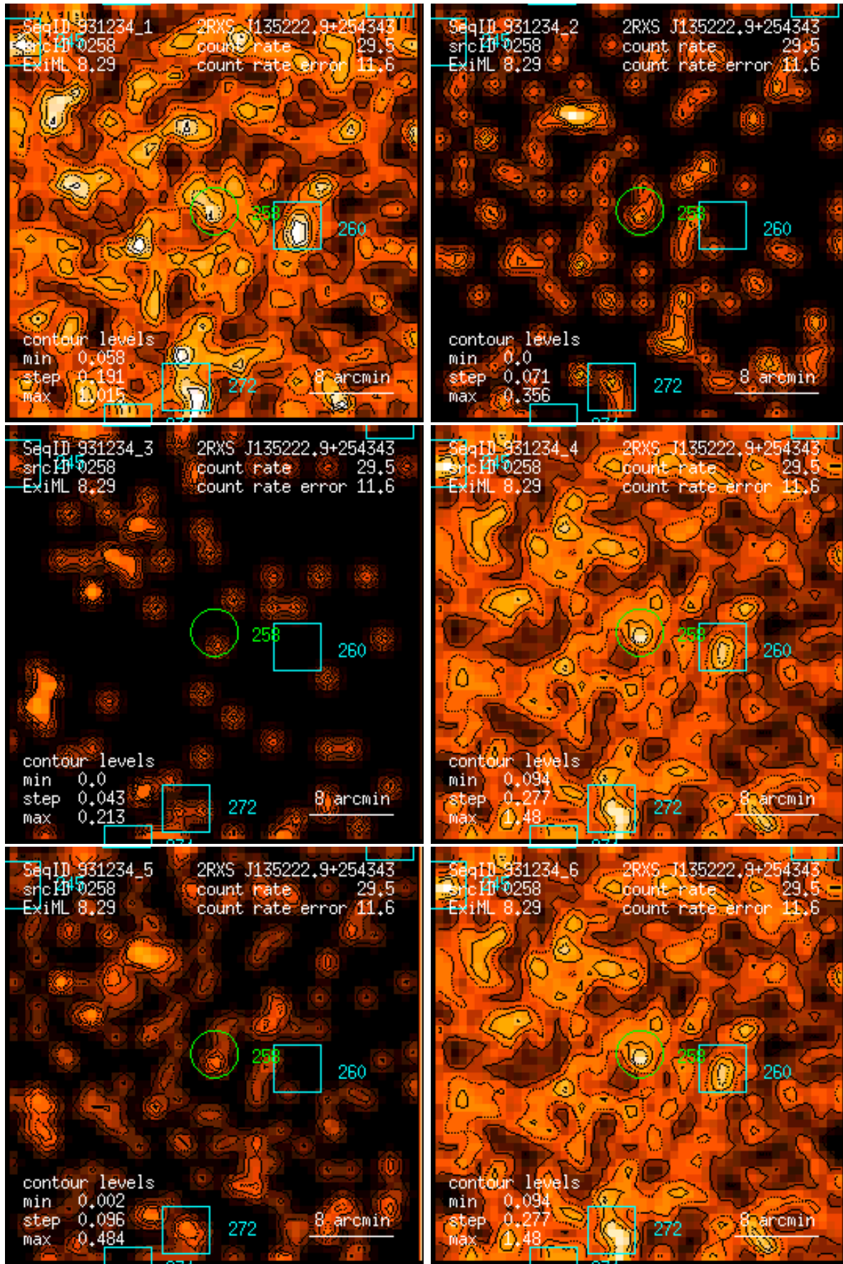
Figure 258: RASS 931234: detection 0258: band rate images, Gaussian filter: (1) PSPC channels 11 – 41, (2) 52 – 90, (3) 91 – 201, (4) 11 – 235, (5) 52 – 201, (6) 11 – 201. Broad band rates in counts/ks. Band rate contour levels in counts/ks/arcmin 2 .
