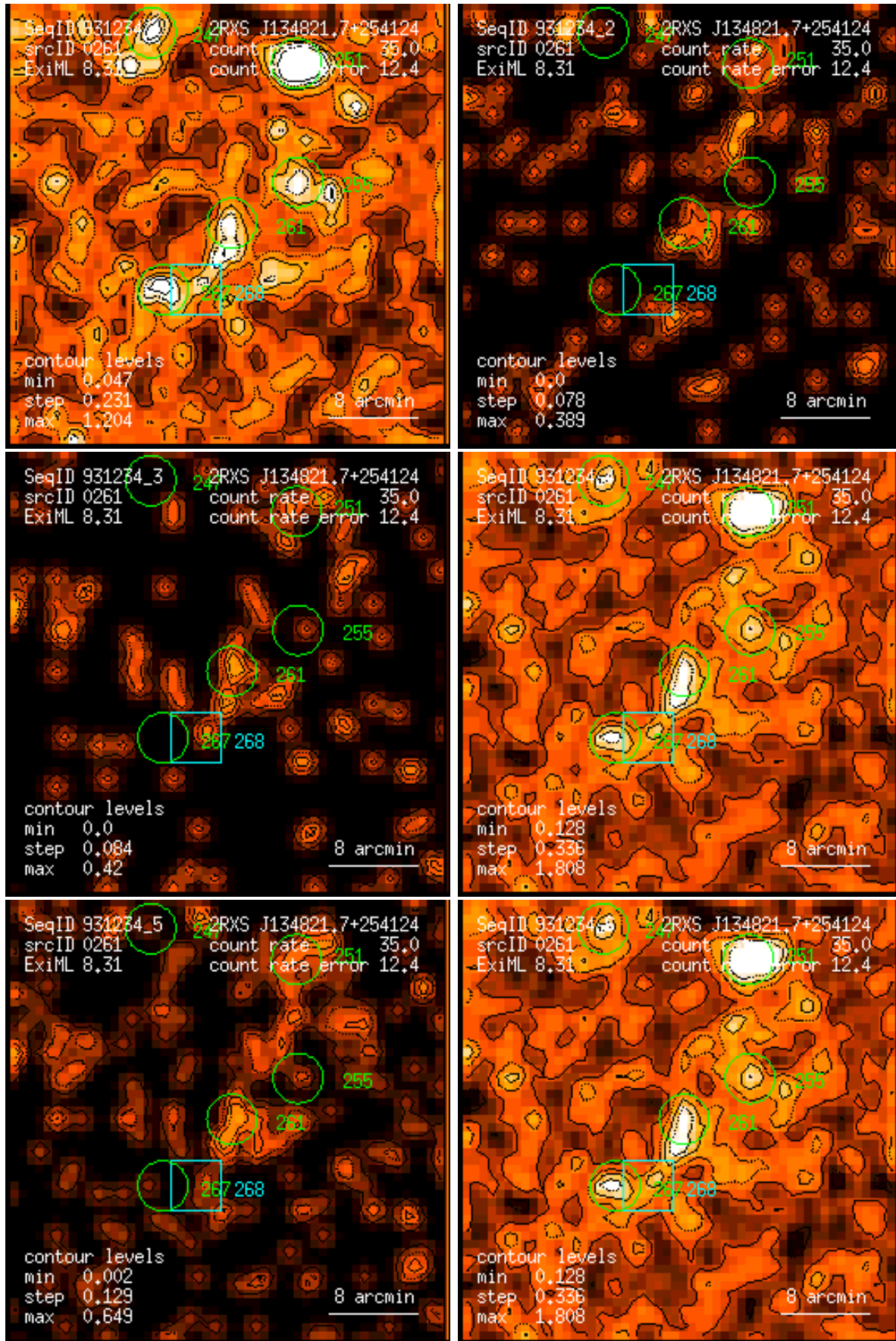
Figure 261: RASS 931234: detection 0261: band rate images, Gaussian filter: (1) PSPC channels 11 – 41, (2) 52 – 90, (3) 91 – 201, (4) 11 – 235, (5) 52 – 201, (6) 11 – 201. Broad band rates in counts/ks. Band rate contour levels in counts/ks/arcmin 2 .
