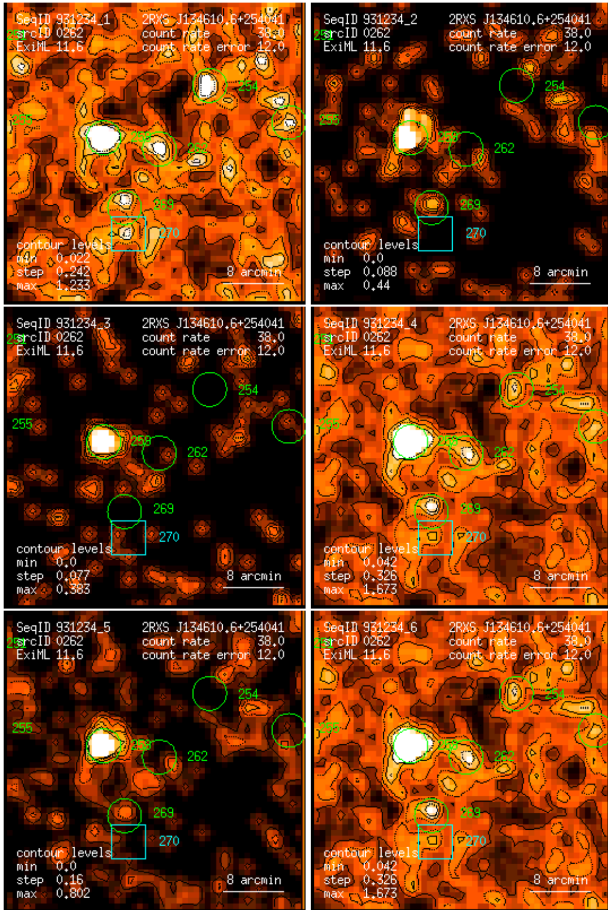
Figure 262: RASS 931234: detection 0262: band rate images, Gaussian filter: (1) PSPC channels 11 – 41, (2) 52 – 90, (3) 91 – 201, (4) 11 – 235, (5) 52 – 201, (6) 11 – 201. Broad band rates in counts/ks. Band rate contour levels in counts/ks/arcmin 2 .
