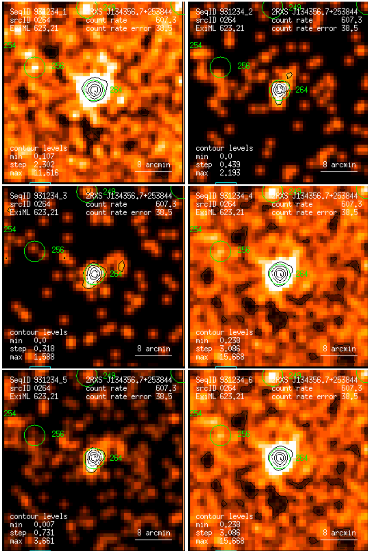
Figure 264: RASS 931234: detection 0264: band rate images, Gaussian filter: (1) PSPC channels 11 – 41, (2) 52 – 90, (3) 91 – 201, (4) 11 – 235, (5) 52 – 201, (6) 11 – 201. Broad band rates in counts/ks. Band rate contour levels in counts/ks/arcmin 2 .
