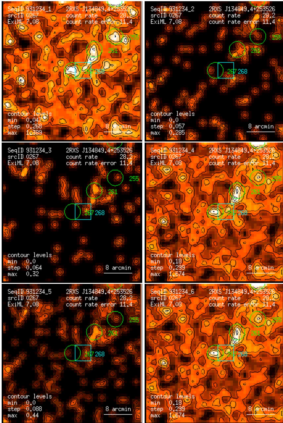
Figure 267: RASS 931234: detection 0267: band rate images, Gaussian filter: (1) PSPC channels 11 – 41, (2) 52 – 90, (3) 91 – 201, (4) 11 – 235, (5) 52 – 201, (6) 11 – 201. Broad band rates in counts/ks. Band rate contour levels in counts/ks/arcmin 2 .
