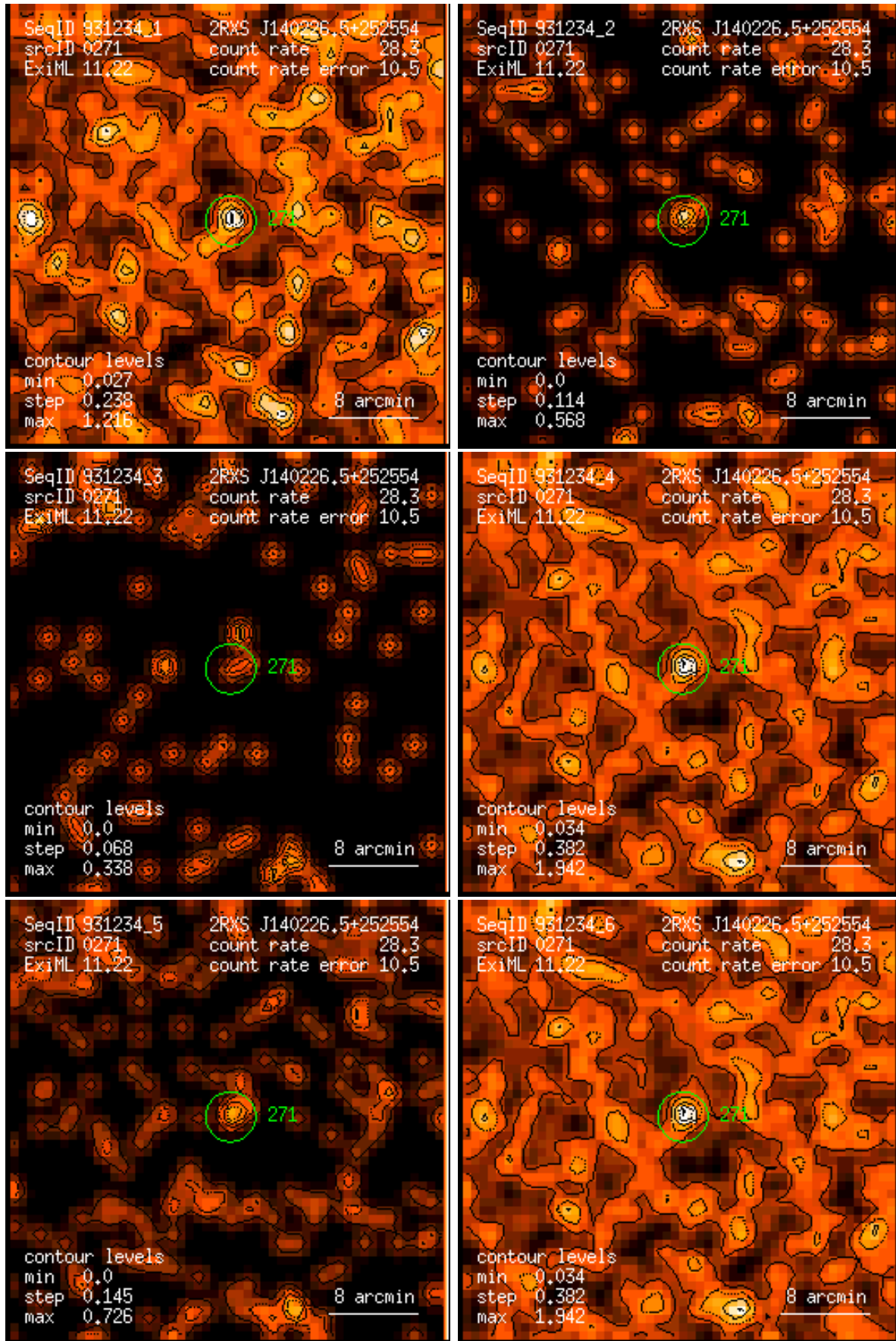
Figure 271: RASS 931234: detection 0271: band rate images, Gaussian filter: (1) PSPC channels 11 – 41, (2) 52 – 90, (3) 91 – 201, (4) 11 – 235, (5) 52 – 201, (6) 11 – 201. Broad band rates in counts/ks. Band rate contour levels in counts/ks/arcmin 2 .
