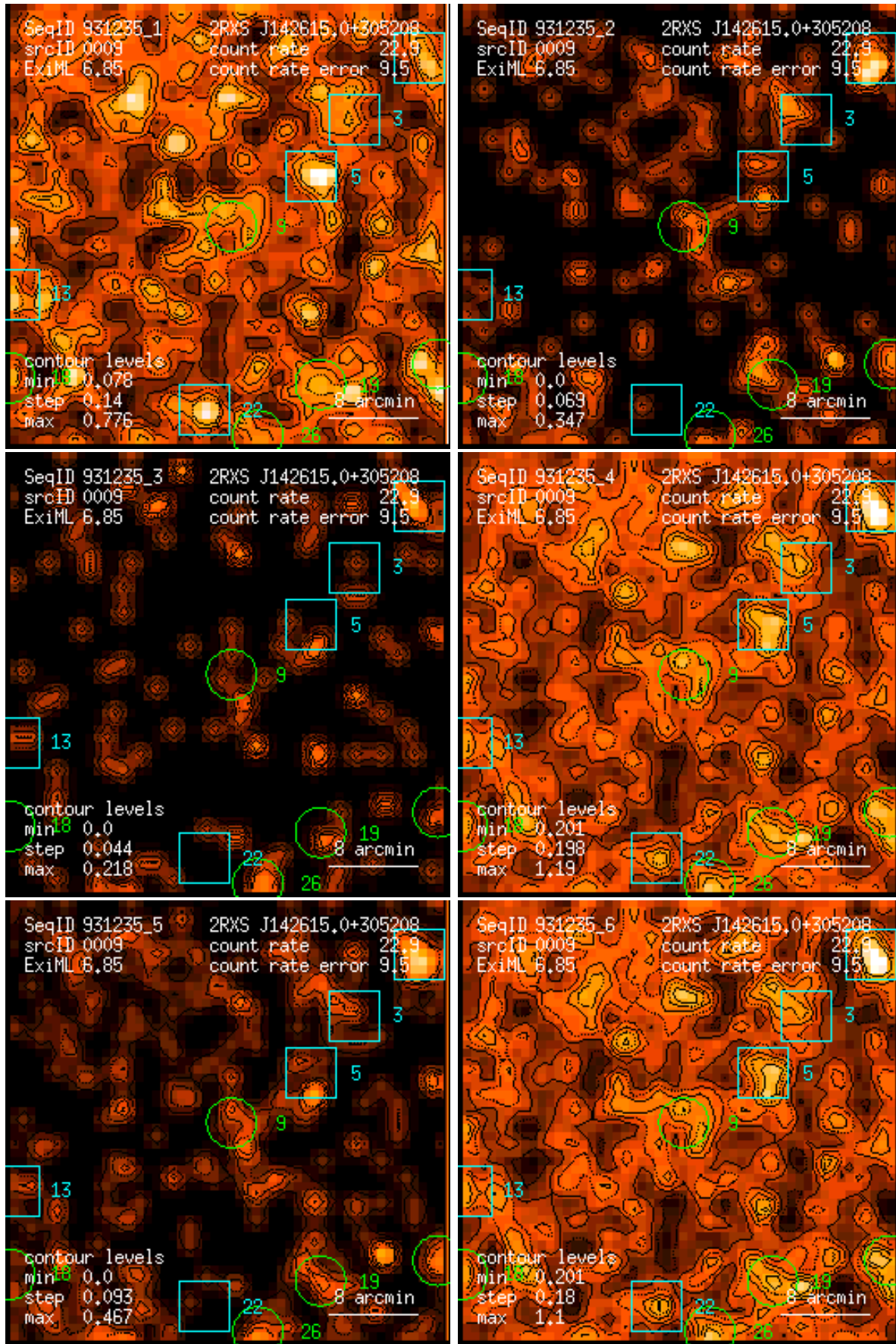
Figure 9: RASS 931235: detection 0009: band rate images, Gaussian filter: (1) PSPC channels 11 – 41, (2) 52 – 90, (3) 91 – 201, (4) 11 – 235, (5) 52 – 201, (6) 11 – 201. Broad band rates in counts/ks. Band rate contour levels in counts/ks/arcmin 2 .
