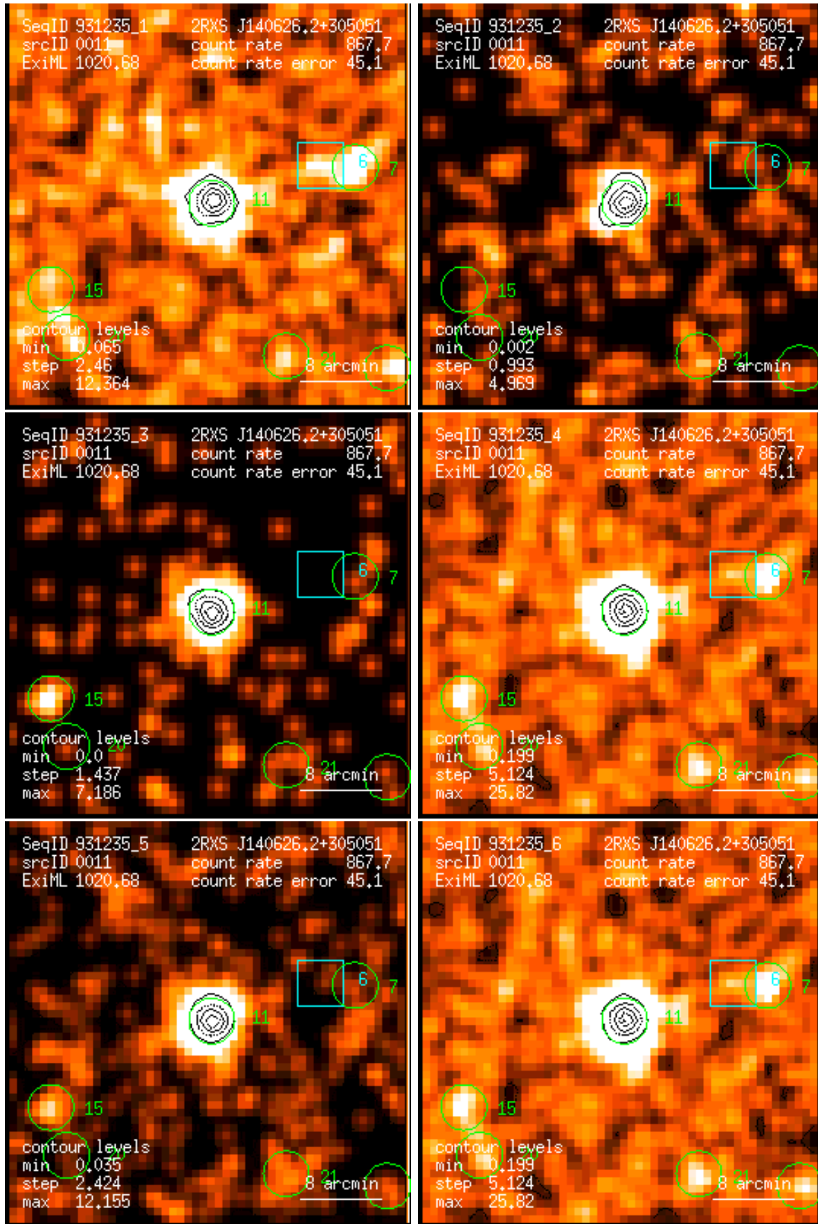
Figure 11: RASS 931235: detection 0011: band rate images, Gaussian filter: (1) PSPC channels 11 – 41, (2) 52 – 90, (3) 91 – 201, (4) 11 – 235, (5) 52 – 201, (6) 11 – 201. Broad band rates in counts/ks. Band rate contour levels in counts/ks/arcmin 2 .
