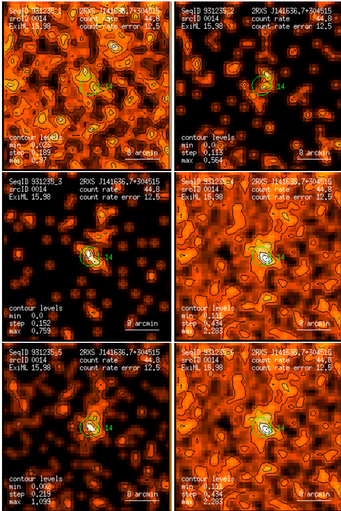
Figure 14: RASS 931235: detection 0014: band rate images, Gaussian filter: (1) PSPC channels 11 – 41, (2) 52 – 90, (3) 91 – 201, (4) 11 – 235, (5) 52 – 201, (6) 11 – 201. Broad band rates in counts/ks. Band rate contour levels in counts/ks/arcmin 2 .
