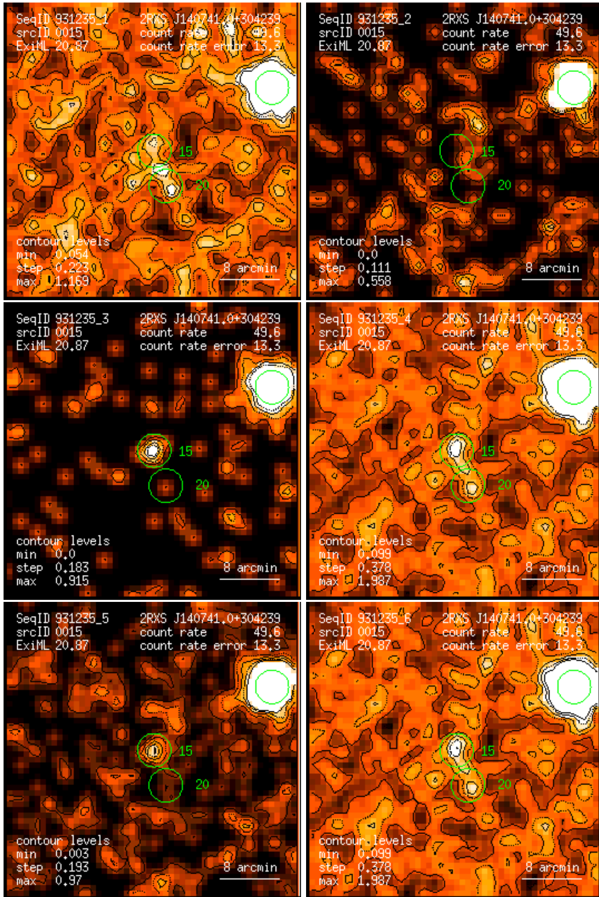
Figure 15: RASS 931235: detection 0015: band rate images, Gaussian filter: (1) PSPC channels 11 – 41, (2) 52 – 90, (3) 91 – 201, (4) 11 – 235, (5) 52 – 201, (6) 11 – 201. Broad band rates in counts/ks. Band rate contour levels in counts/ks/arcmin 2 .
