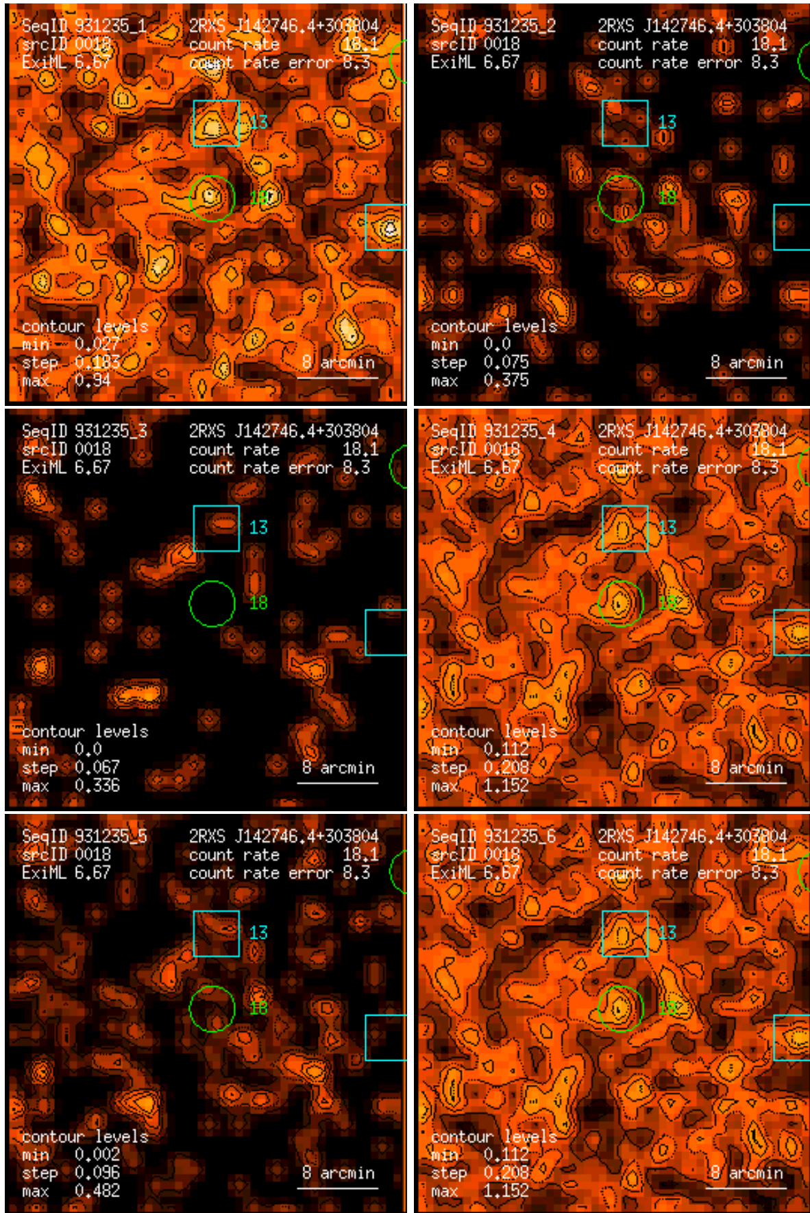
Figure 18: RASS 931235: detection 0018: band rate images, Gaussian filter: (1) PSPC channels 11 – 41, (2) 52 – 90, (3) 91 – 201, (4) 11 – 235, (5) 52 – 201, (6) 11 – 201. Broad band rates in counts/ks. Band rate contour levels in counts/ks/arcmin 2 .
