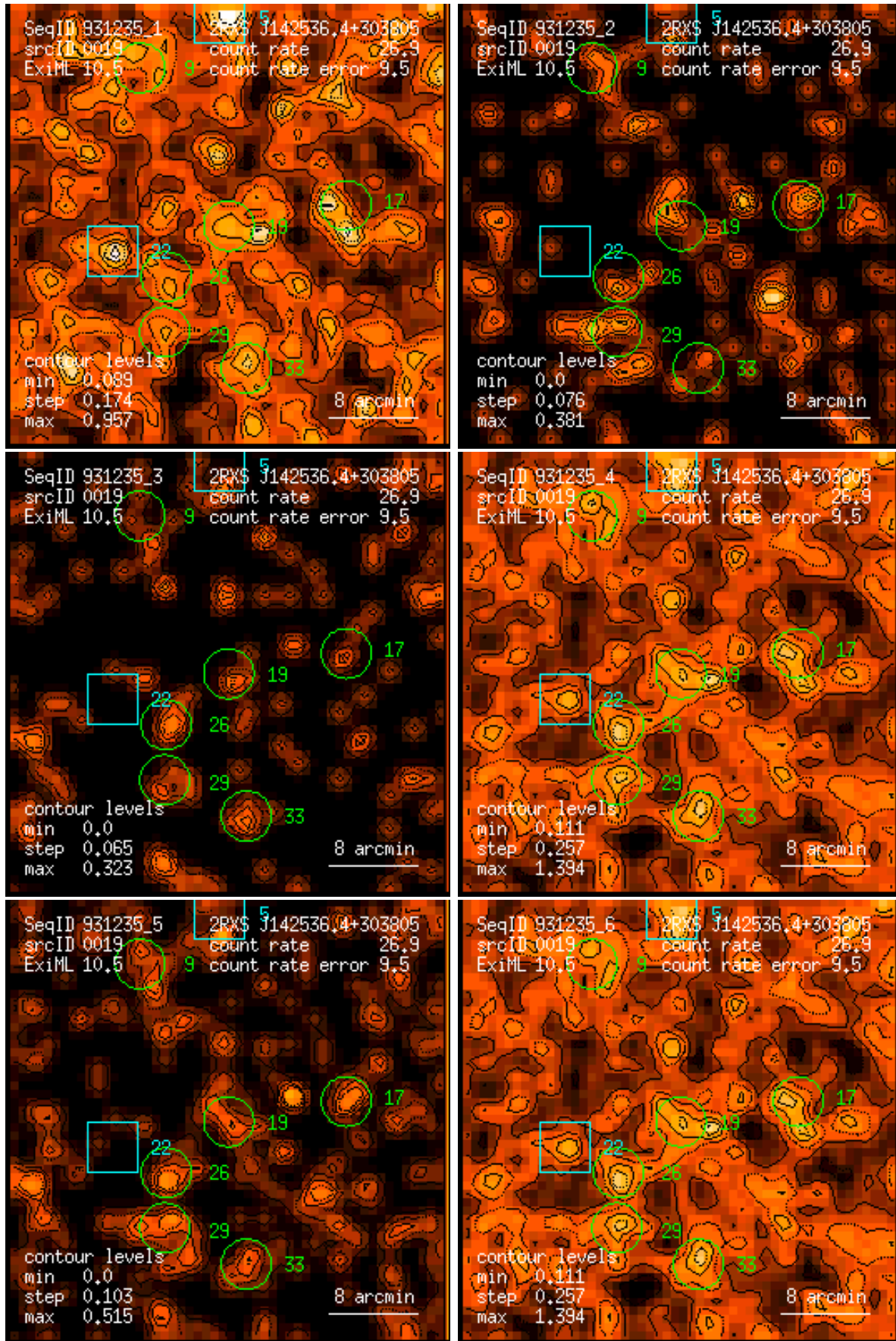
Figure 19: RASS 931235: detection 0019: band rate images, Gaussian filter: (1) PSPC channels 11 – 41, (2) 52 – 90, (3) 91 – 201, (4) 11 – 235, (5) 52 – 201, (6) 11 – 201. Broad band rates in counts/ks. Band rate contour levels in counts/ks/arcmin 2 .
