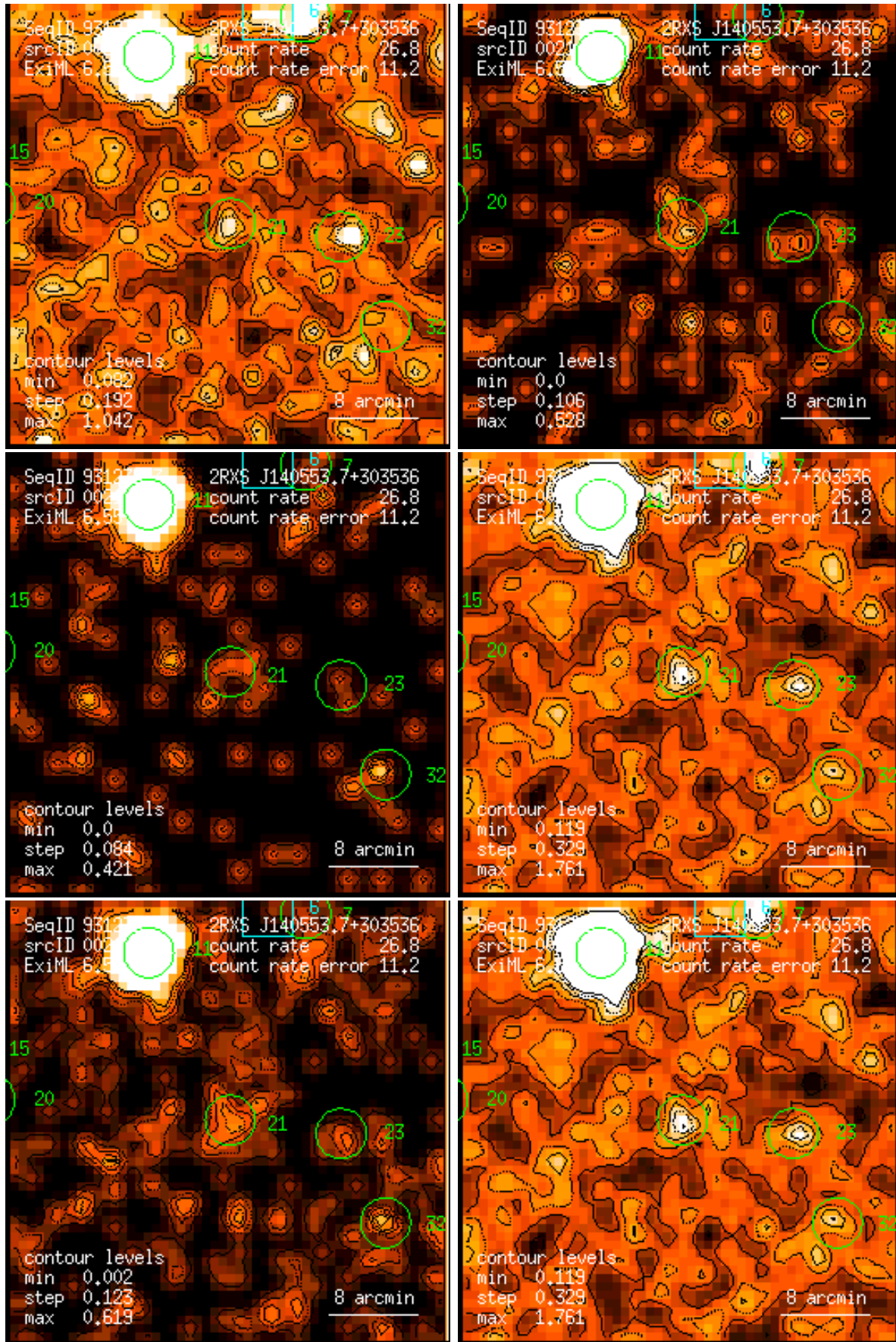
Figure 21: RASS 931235: detection 0021: band rate images, Gaussian filter: (1) PSPC channels 11 – 41, (2) 52 – 90, (3) 91 – 201, (4) 11 – 235, (5) 52 – 201, (6) 11 – 201. Broad band rates in counts/ks. Band rate contour levels in counts/ks/arcmin 2 .
