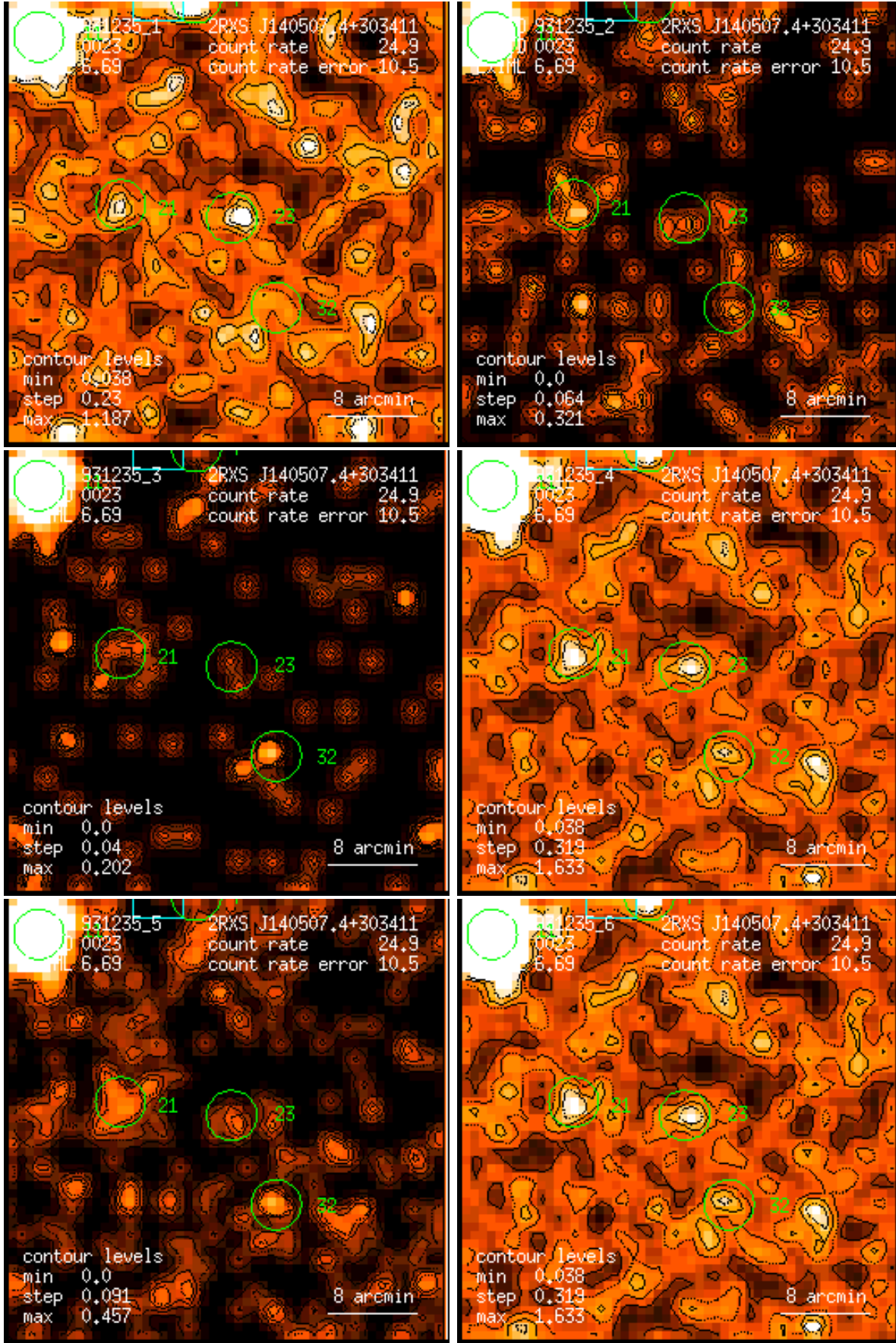
Figure 23: RASS 931235: detection 0023: band rate images, Gaussian filter: (1) PSPC channels 11 – 41, (2) 52 – 90, (3) 91 – 201, (4) 11 – 235, (5) 52 – 201, (6) 11 – 201. Broad band rates in counts/ks. Band rate contour levels in counts/ks/arcmin 2 .
