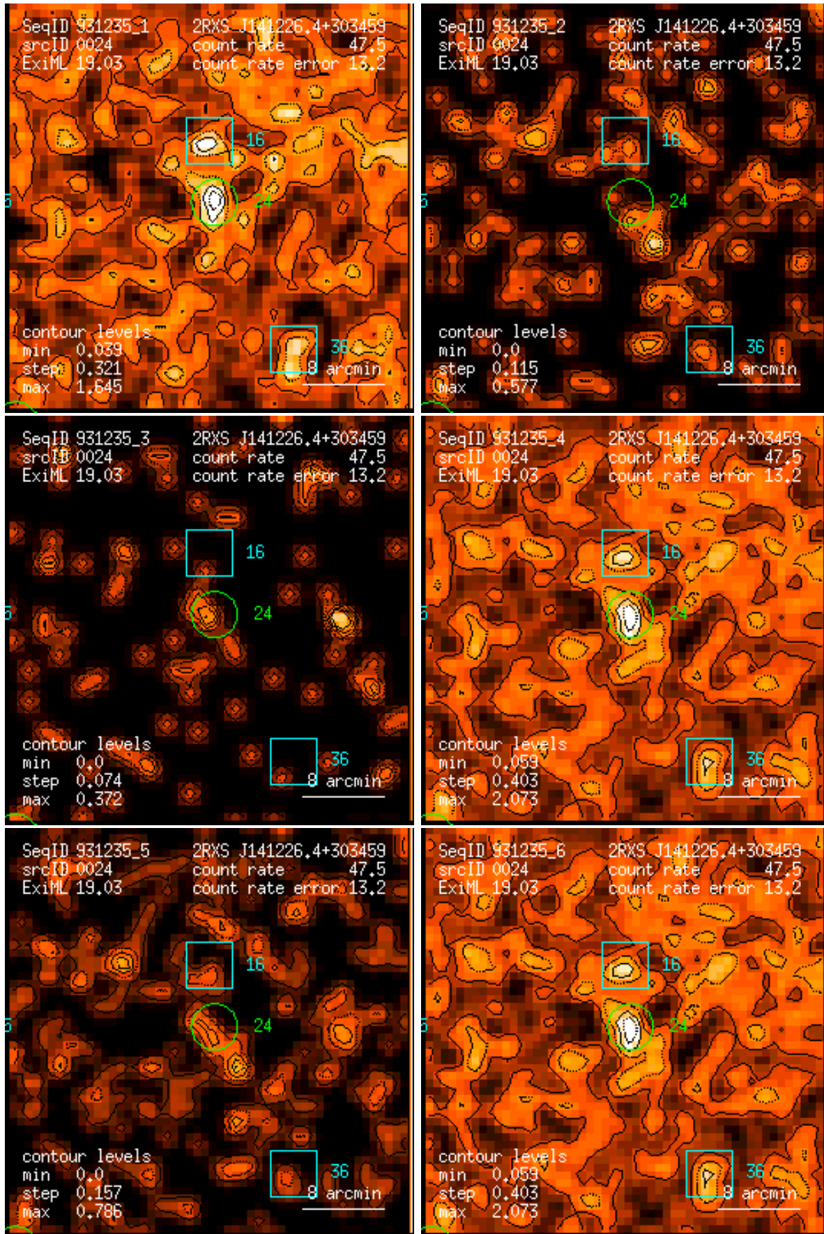
Figure 24: RASS 931235: detection 0024: band rate images, Gaussian filter: (1) PSPC channels 11 – 41, (2) 52 – 90, (3) 91 – 201, (4) 11 – 235, (5) 52 – 201, (6) 11 – 201. Broad band rates in counts/ks. Band rate contour levels in counts/ks/arcmin 2 .
