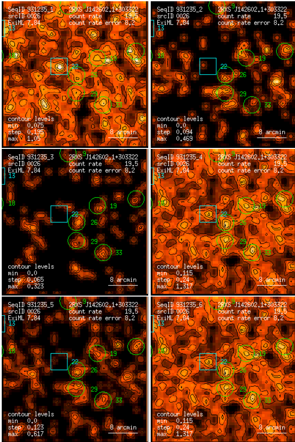
Figure 26: RASS 931235: detection 0026: band rate images, Gaussian filter: (1) PSPC channels 11 – 41, (2) 52 – 90, (3) 91 – 201, (4) 11 – 235, (5) 52 – 201, (6) 11 – 201. Broad band rates in counts/ks. Band rate contour levels in counts/ks/arcmin 2 .
