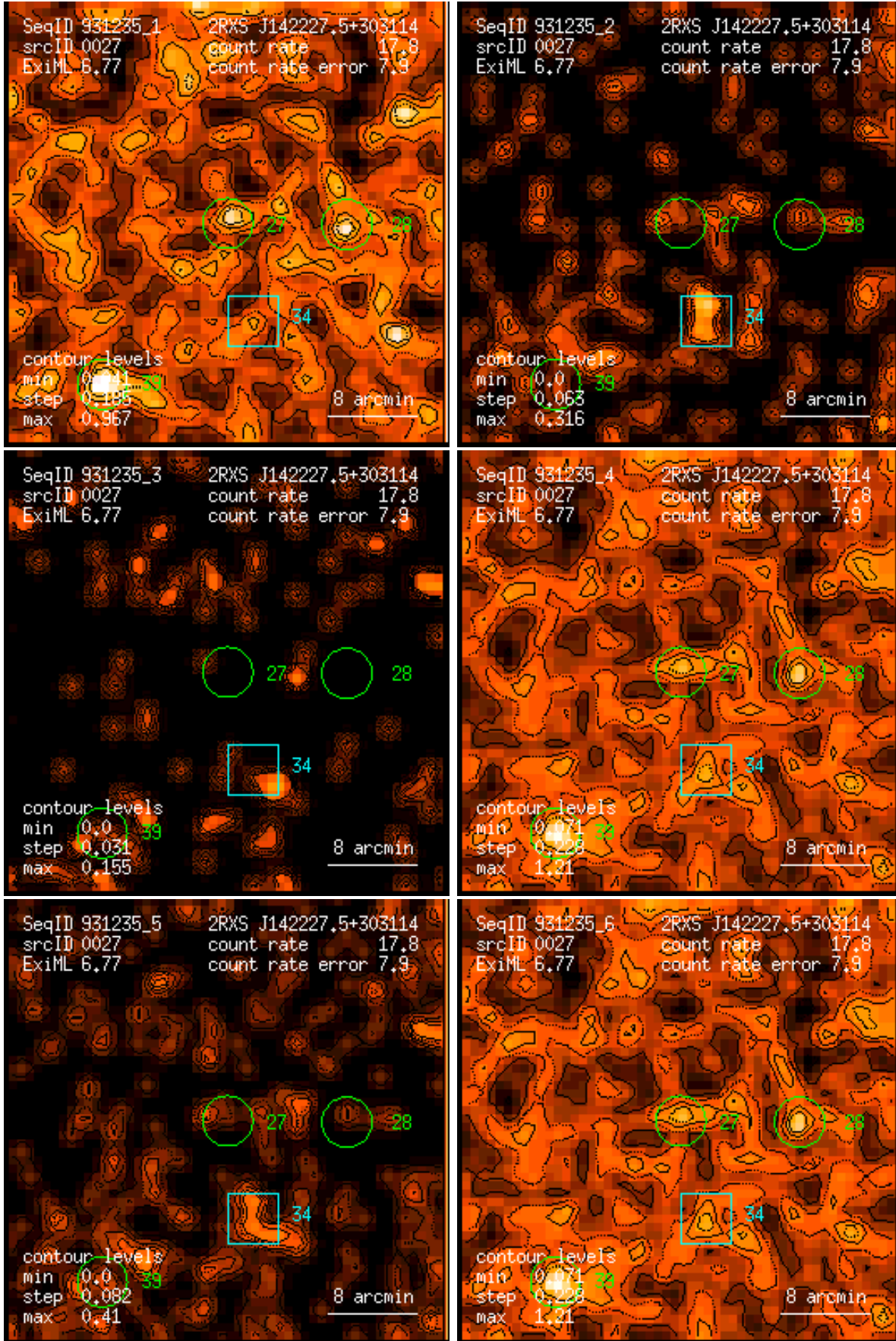
Figure 27: RASS 931235: detection 0027: band rate images, Gaussian filter: (1) PSPC channels 11 – 41, (2) 52 – 90, (3) 91 – 201, (4) 11 – 235, (5) 52 – 201, (6) 11 – 201. Broad band rates in counts/ks. Band rate contour levels in counts/ks/arcmin 2 .
