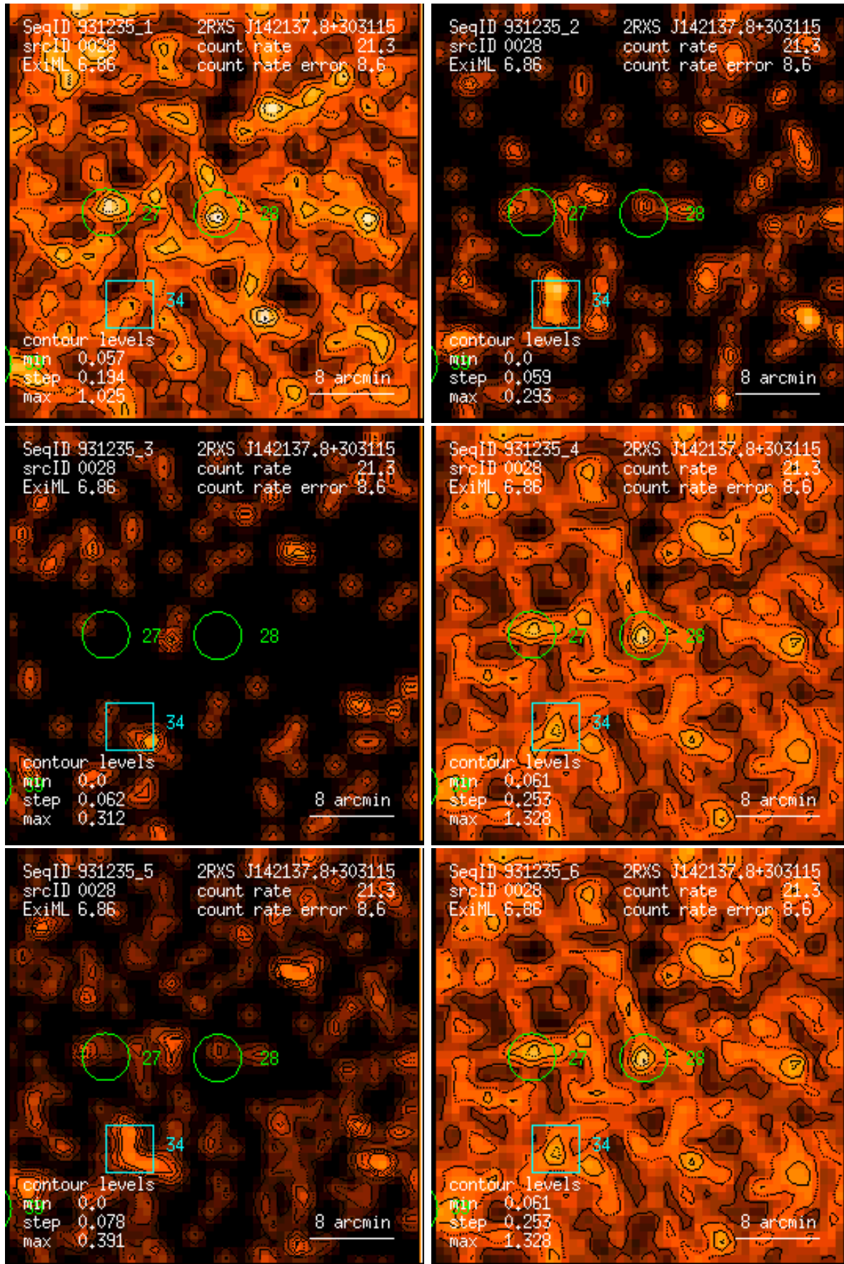
Figure 28: RASS 931235: detection 0028: band rate images, Gaussian filter: (1) PSPC channels 11 – 41, (2) 52 – 90, (3) 91 – 201, (4) 11 – 235, (5) 52 – 201, (6) 11 – 201. Broad band rates in counts/ks. Band rate contour levels in counts/ks/arcmin 2 .
