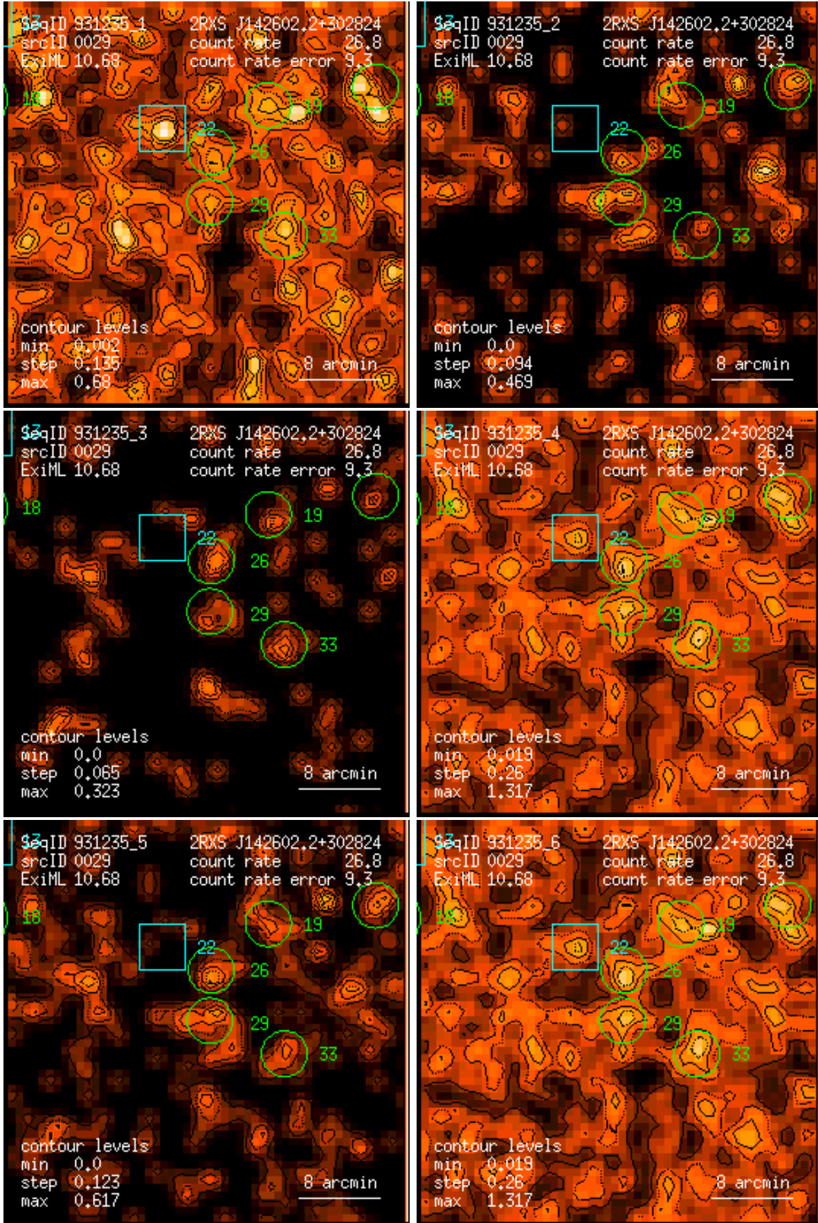
Figure 29: RASS 931235: detection 0029: band rate images, Gaussian filter: (1) PSPC channels 11 – 41, (2) 52 – 90, (3) 91 – 201, (4) 11 – 235, (5) 52 – 201, (6) 11 – 201. Broad band rates in counts/ks. Band rate contour levels in counts/ks/arcmin 2 .
