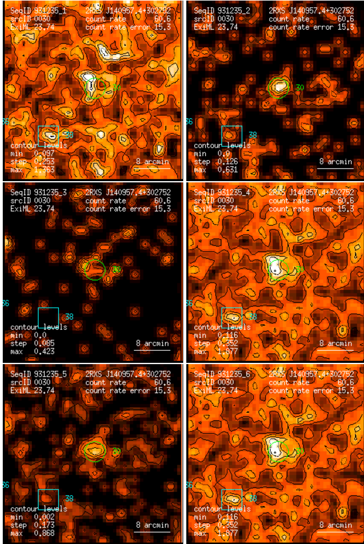
Figure 30: RASS 931235: detection 0030: band rate images, Gaussian filter: (1) PSPC channels 11 – 41, (2) 52 – 90, (3) 91 – 201, (4) 11 – 235, (5) 52 – 201, (6) 11 – 201. Broad band rates in counts/ks. Band rate contour levels in counts/ks/arcmin 2 .
