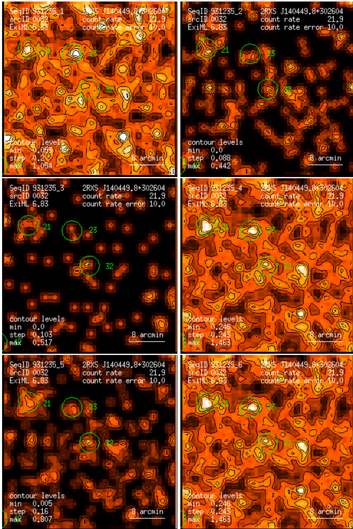
Figure 32: RASS 931235: detection 0032: band rate images, Gaussian filter: (1) PSPC channels 11 – 41, (2) 52 – 90, (3) 91 – 201, (4) 11 – 235, (5) 52 – 201, (6) 11 – 201. Broad band rates in counts/ks. Band rate contour levels in counts/ks/arcmin 2 .
