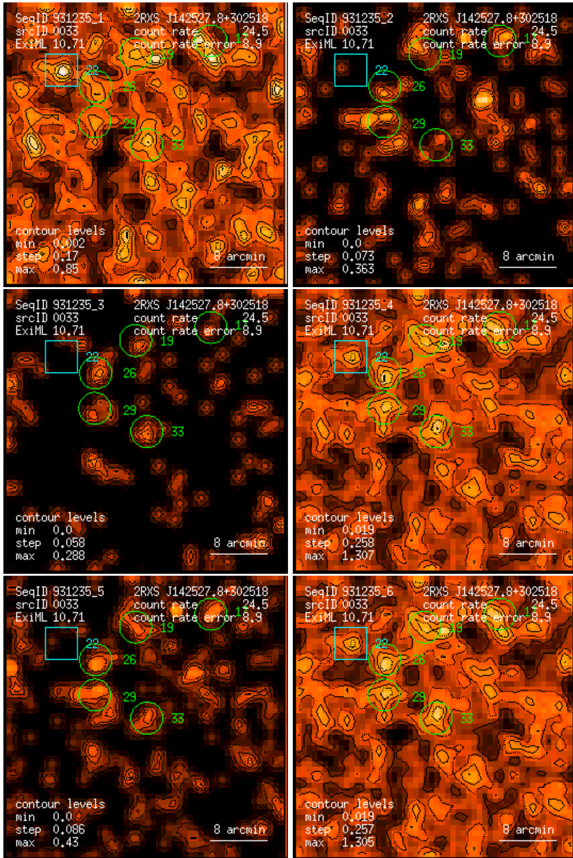
Figure 33: RASS 931235: detection 0033: band rate images, Gaussian filter: (1) PSPC channels 11 – 41, (2) 52 – 90, (3) 91 – 201, (4) 11 – 235, (5) 52 – 201, (6) 11 – 201. Broad band rates in counts/ks. Band rate contour levels in counts/ks/arcmin 2 .
