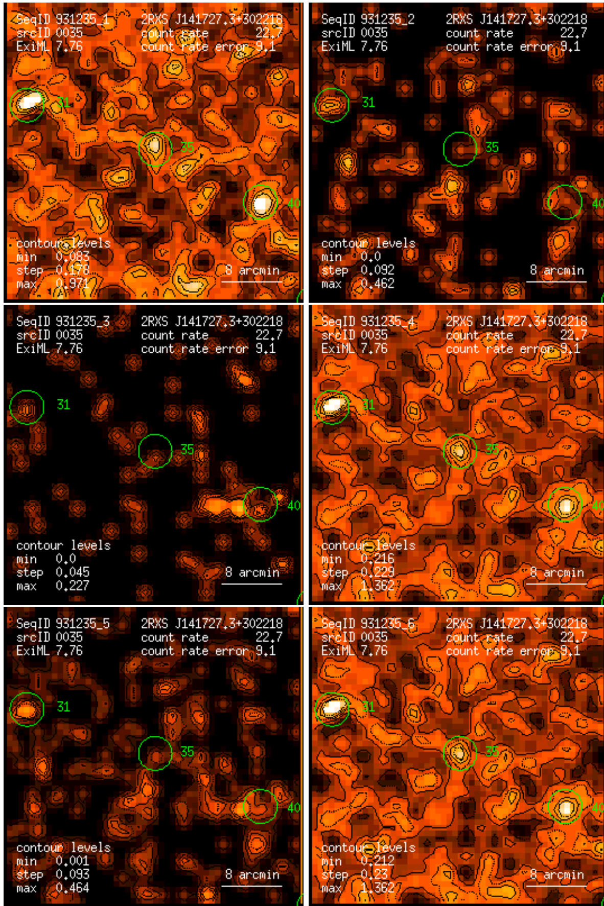
Figure 35: RASS 931235: detection 0035: band rate images, Gaussian filter: (1) PSPC channels 11 – 41, (2) 52 – 90, (3) 91 – 201, (4) 11 – 235, (5) 52 – 201, (6) 11 – 201. Broad band rates in counts/ks. Band rate contour levels in counts/ks/arcmin 2 .
