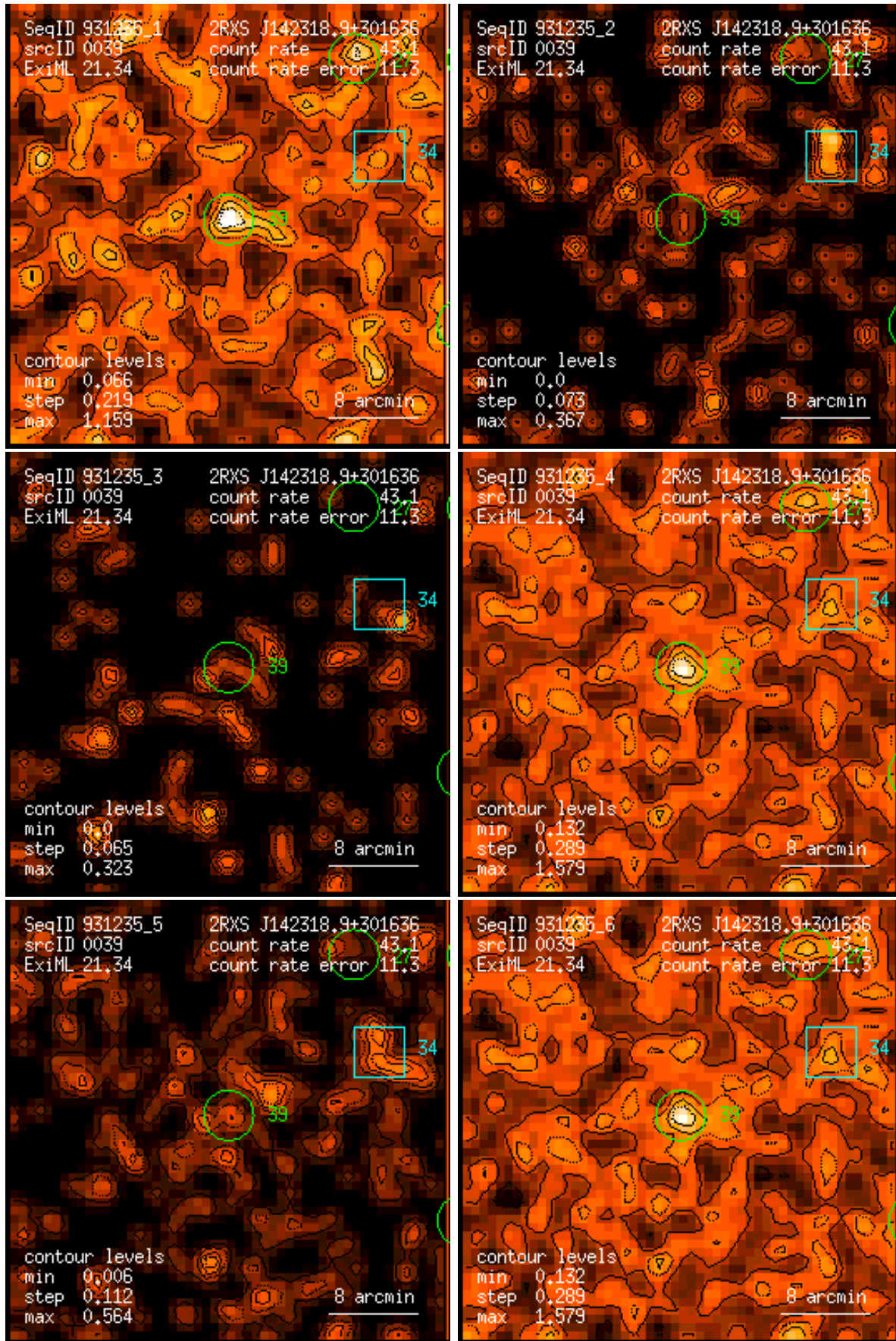
Figure 39: RASS 931235: detection 0039: band rate images, Gaussian filter: (1) PSPC channels 11 – 41, (2) 52 – 90, (3) 91 – 201, (4) 11 – 235, (5) 52 – 201, (6) 11 – 201. Broad band rates in counts/ks. Band rate contour levels in counts/ks/arcmin 2 .
